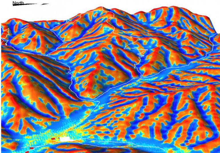
GRASS Example Image: Surface Curvatures
