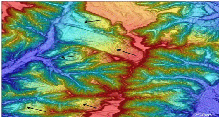
Figure 5. Landslide topography of Chuetsu-district in Niigata
