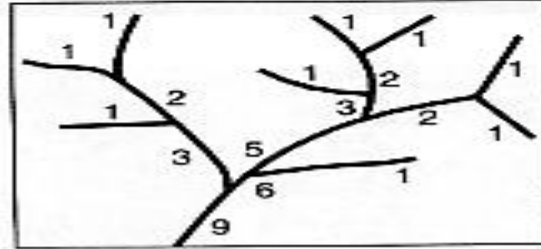
Shreve (1967)
