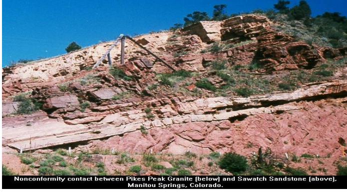
Nonconformity contact between Pikes Peak Granite (below) and Sawatch Sandstone (above), Manitou Springs, Colorado.
