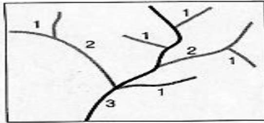
Horton (1945)
