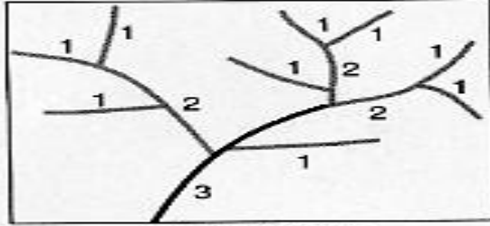
Strahler (1952)
