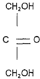
Dihydroxy acetone
