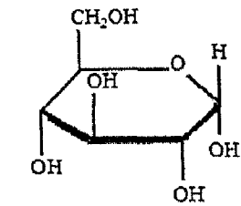
\alpha -D- Glucopyranose
