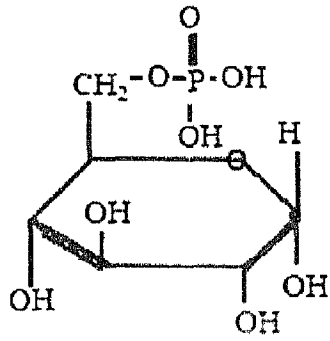
Glucose - -6-Phosphate
