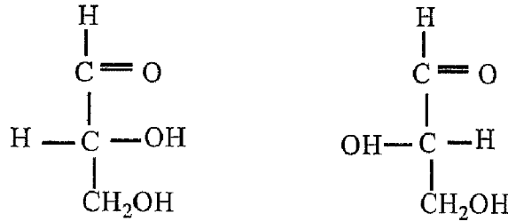
D-glyceraldehyde
