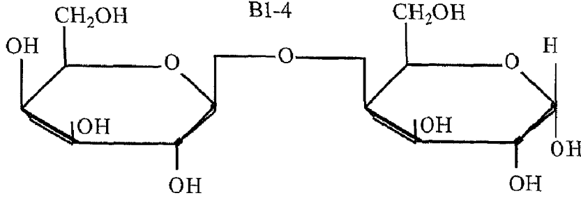
\alpha - Lactose
