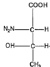
L -Allo threonine
