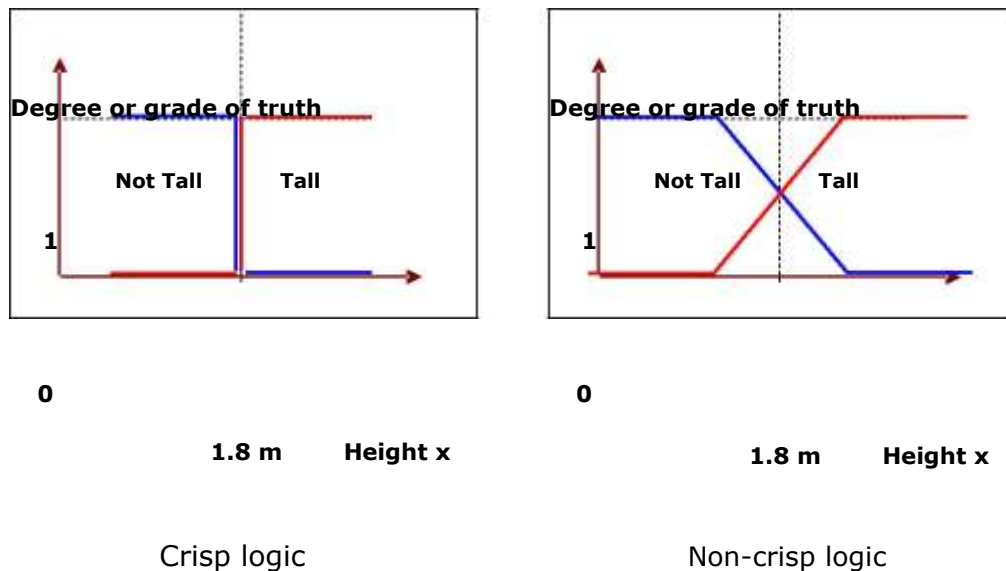
Fig. 1 Set Representation – Degree or grade of truth
