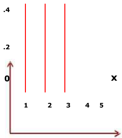
Fig Fuzzy plot of 1st projection R^{(1)} Fig Fuzzy plot of 2nd projection R^{(2)}
