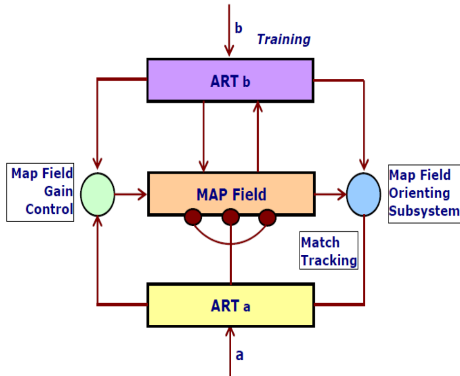
Fig. Supervised ARTMAP system
