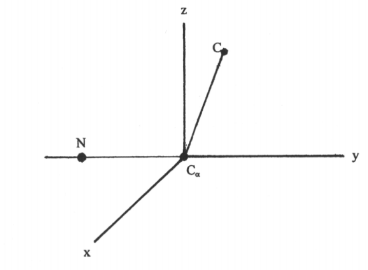
Figure 5-14. Locations of protein backbone atoms.
