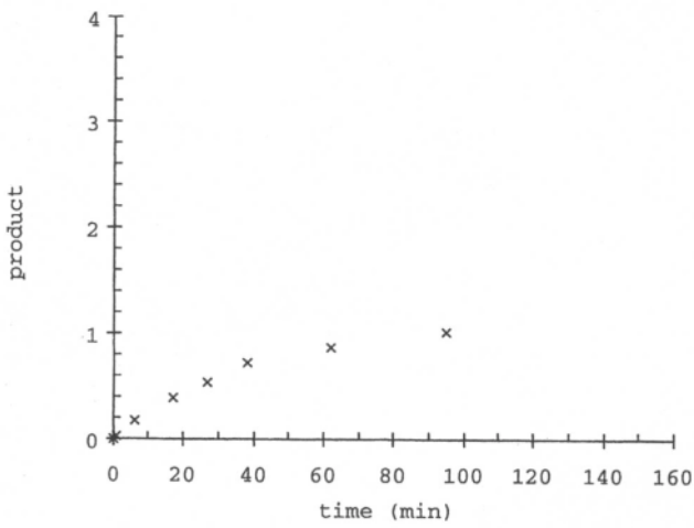
Figure 4-14. Plot of product against time for [S]_0 = 0.0208 \text{ n.}
