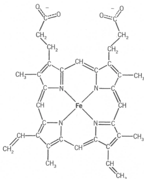
Figure 2-1. The heme.
