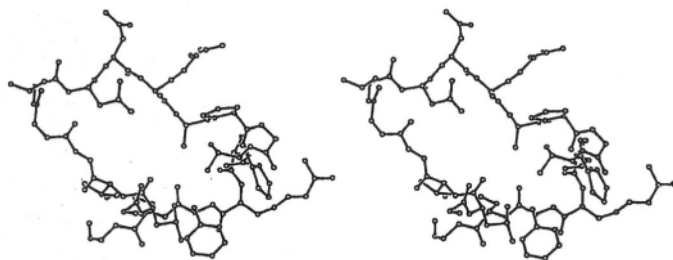
Figure 6-16. Stereo view of CDRL2 of MOPC104E.
