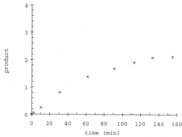
Figure 4-13. Plot of product against time for [S]_0 = 0.0416 \text{ n.}
