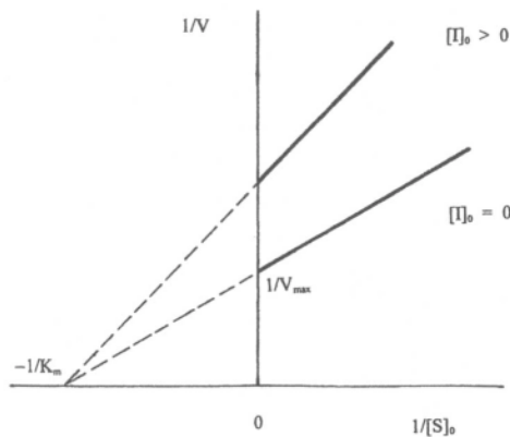
Figure. 4-19. Non-competitive inhibitor.
