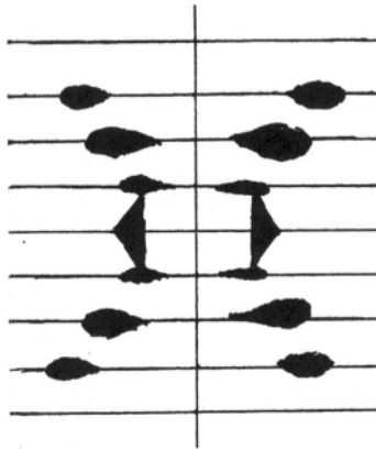
Figure 8-1. Sketch of the fiber X-ray diffraction picture of the sodium salt of DNA obtained Franklin and Gosling (1953), including only up to the fourth layer line.
