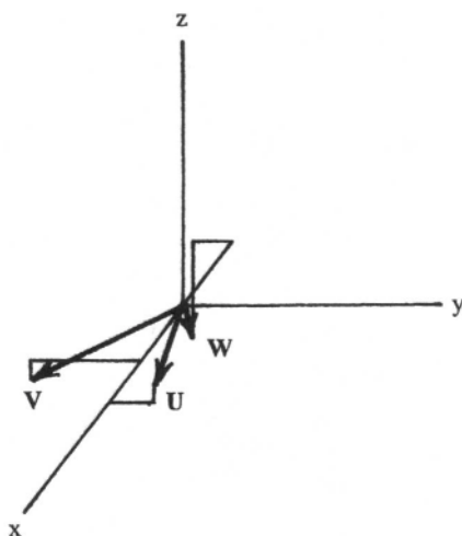
Figure 5-7. Unit vectors \mathbf{U} , \mathbf{V} and \mathbf{W} to the three planes illustrated in Fig. 5-3.
