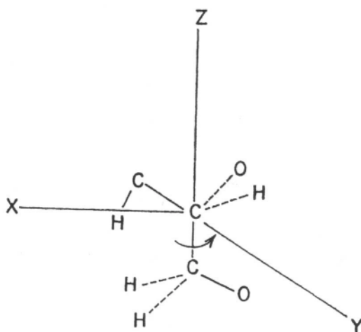
Figure 7-5. Definition of \theta_2 , rotation around C_4'-C_5' bond.
