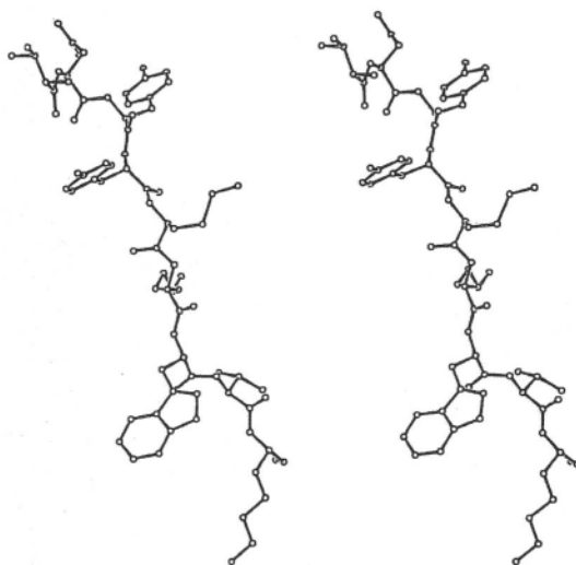
Figure 6-14. Stereo view of CDRH1 of MOPC104E.
