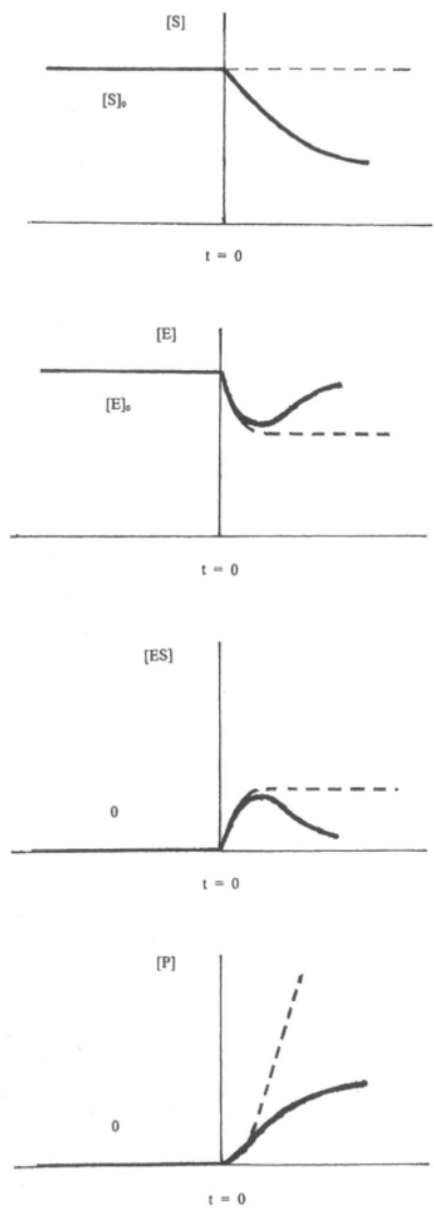
Figure 4-17. Schematic time courses of [S] , [E] , [ES] and [P] for low [S]_0 .
