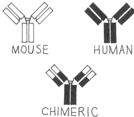
Figure 1-14. Schematic representation of a chimeric antibody.
