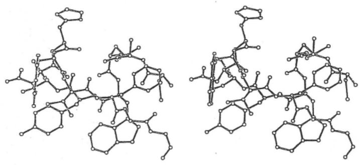
Figure 6-12. Stereo view of CDRL3 of MOPC104E.
