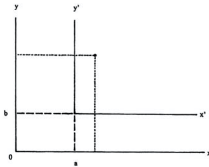
Figure A-1. Translation of coordinates in two dimension.
