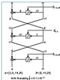
Figure 12.9 A 3-round linear approximation for DES.
