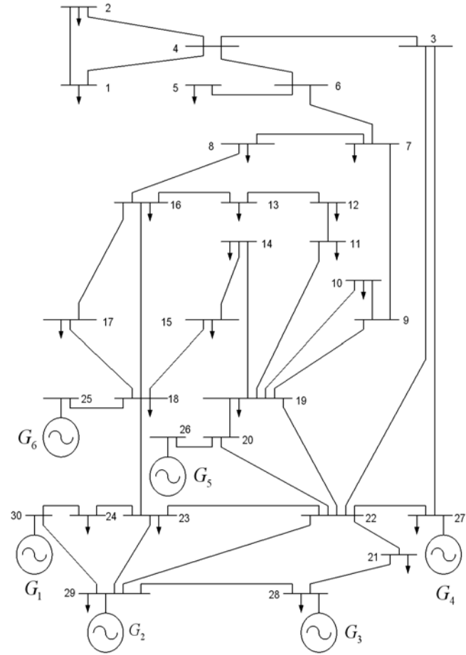
Fig. 5 Single-line diagram of the test system
