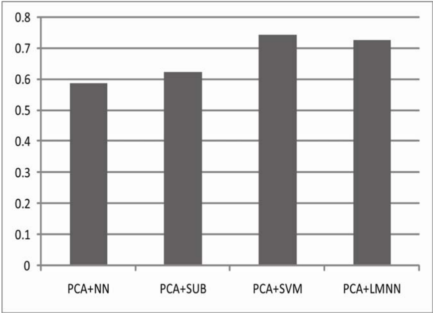
Fig. 10 Comparison of single classifier performance averaged across all six trait dimensions
