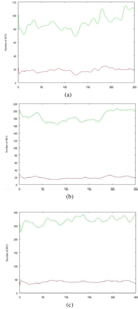
Fig. 9 Number of MCCs along time for the 3 testing sequence, red lines for Algorithm 1; green lines for Algorithm 2 (From top to bottom: sequence 1, sequence 2 and sequence 3). Algorithm 3 detects much more MCCs for all of the three video sequences
