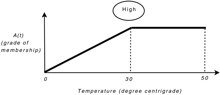
Fig. 1 Membership function
