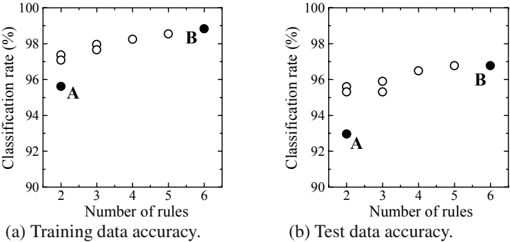
Fig. 10 Obtained non-dominated fuzzy rule-based classifiers (Breast W)
