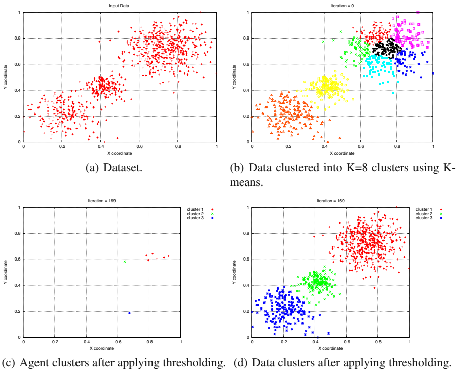
Fig. 11 Stable output of (K-means+FClust) hybrid on a 3 cluster-data set where sim_{th}=0.73 (using Eqn.(2)), d_{th}=1.0 . d_{ideal\_h} for FClust=0.04, d_{ideal\_h} for cluster forming =0.08.
