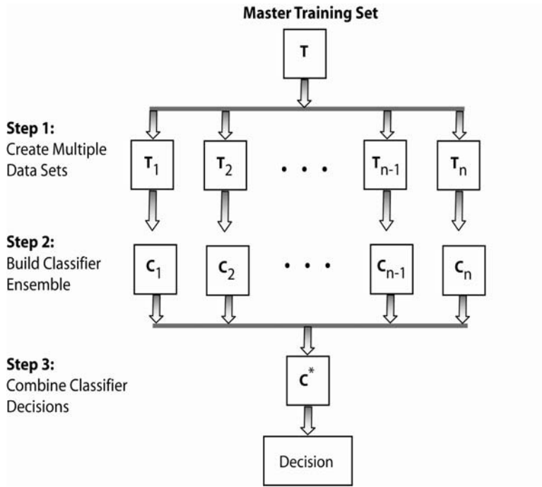
Fig. 3 General schematic of classifier ensembles
