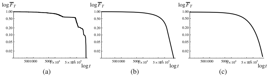
Fig. 6 CCDF LogLogPlot of a T randomly varying according to: (a) the Cambridge/Haggle Crawdad dataset; and (b) a double Pareto law; and (c) a power law followed by an exponential one
