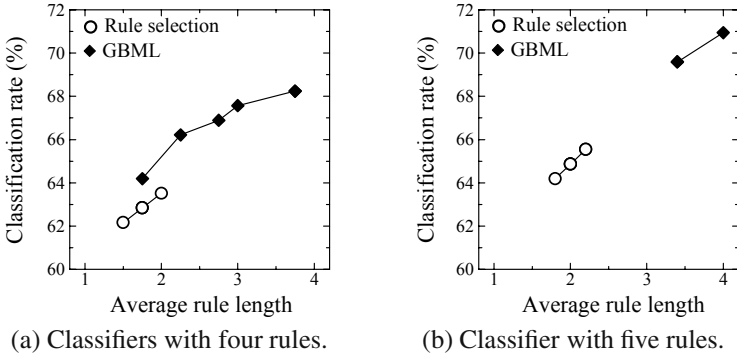
Fig. 30 Relation between the accuracy and the average rule length (Heart C)
