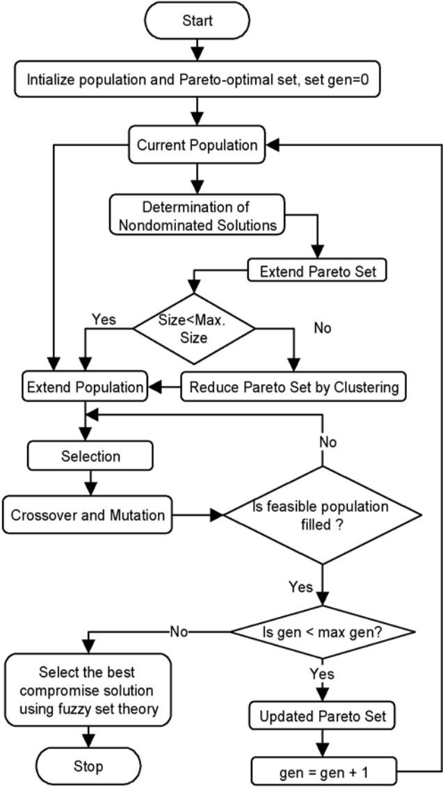
Fig. 4 Computational flow of the developed SPEA
