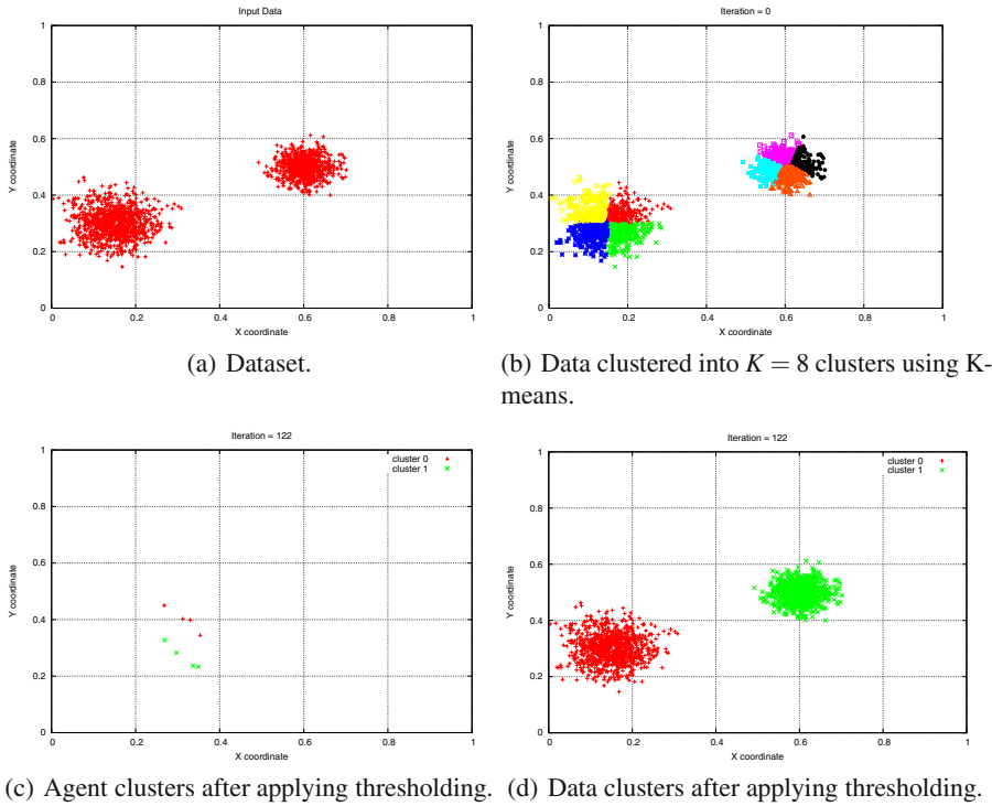
Fig. 10 Stable output of (K-means+FClust) hybrid on a 2 cluster-data set where sim_{th}=0.88 (using Eqn.(2)), d_{th}=0.4 . d_{ideal\_h} for FClust=0.04, d_{ideal\_h} for forming clusters = 0.08
