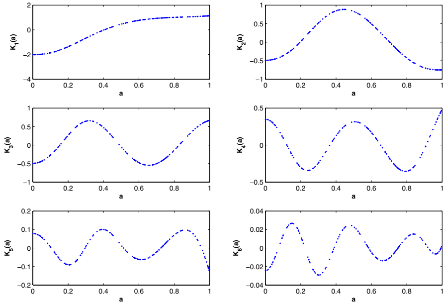
Fig. 1 The curves \mathcal{C}_{\mathbf{y}}^j(\mathbf{x}) described by the components k_j(\mathbf{x}) , for j = 1, \dots, 6 of a Duffing ordinary differential equation
