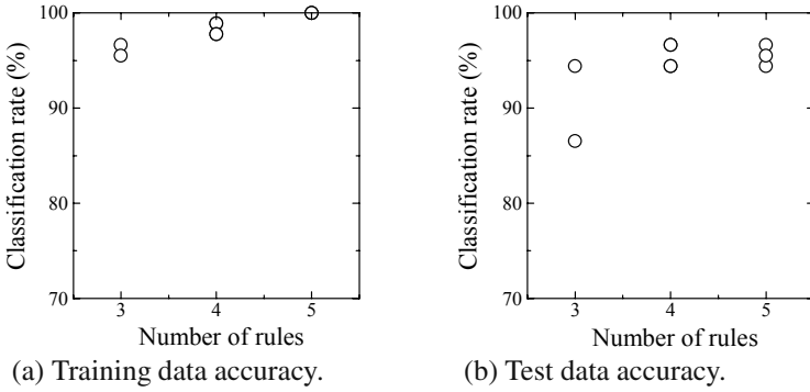
Fig. 29 Obtained non-dominated fuzzy rule-based classifiers (Wine)
