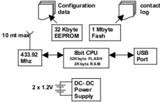
Fig. 7 PTR architecture
