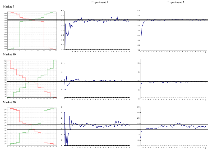
Fig. 2 Agent-Based Double Auction Market Simulation with GP Agents. The three markets presented here are selected and adapted from [26], Fig. 4
