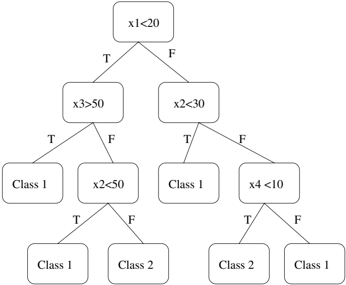
Fig. 1 An example of a decision tree
