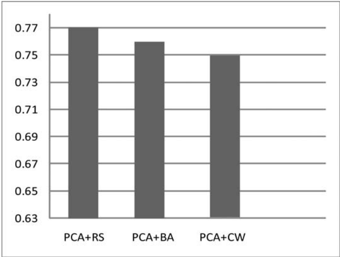
Fig. 12 Comparison of ensemble classifier performance averaged across all six trait dimensions
