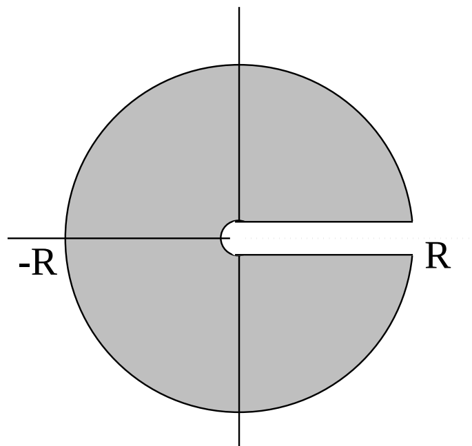
Figure 6.3: A contour for z^q , 0 < q < 1 .
