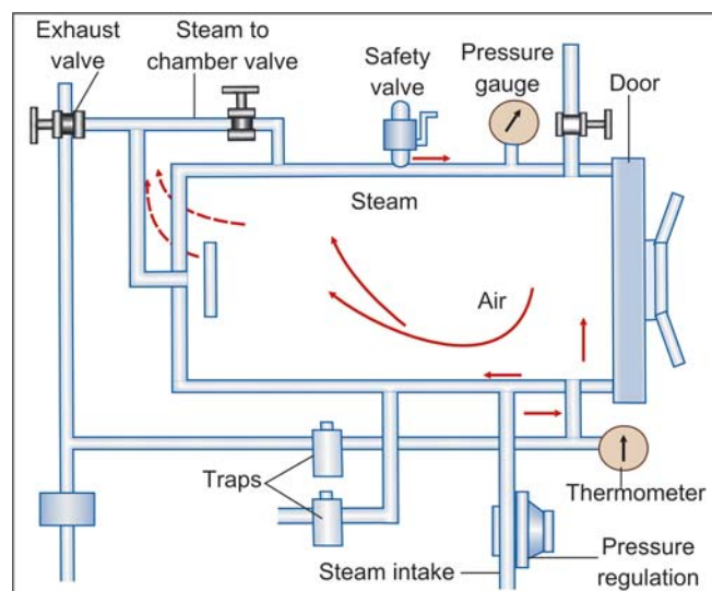
Fig. 9-2. Steam autoclave
