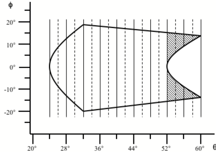
Figure 7.2: A rectangular particle detector has a non-azimuthally symmetric shape in the \theta, \phi space of projectile scattering angle. This shape must be defined by entering a number ( NFI ) of azimuthal angular ranges. In the hatched region, NFI = 2 ranges must be entered specifying the two active regions. The solid lines represent \theta meshpoints, while the dashed lines indicate \theta subdivisions. The rapid variation in active \phi range in the hatched region necessitates input of the active ranges of \Delta\phi at each subdivision specifying each of the two active detection regions shown hatched.
