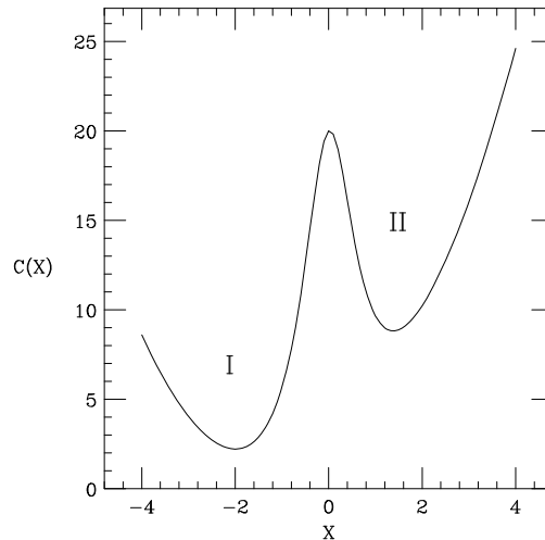
Figure 13.1: An example of a function which can cause difficulties with strict minimization procedures. A procedure using a starting value of x in region “II” ( x > 0 ) will not converge to the global minimum at x \approx -2.0 .
