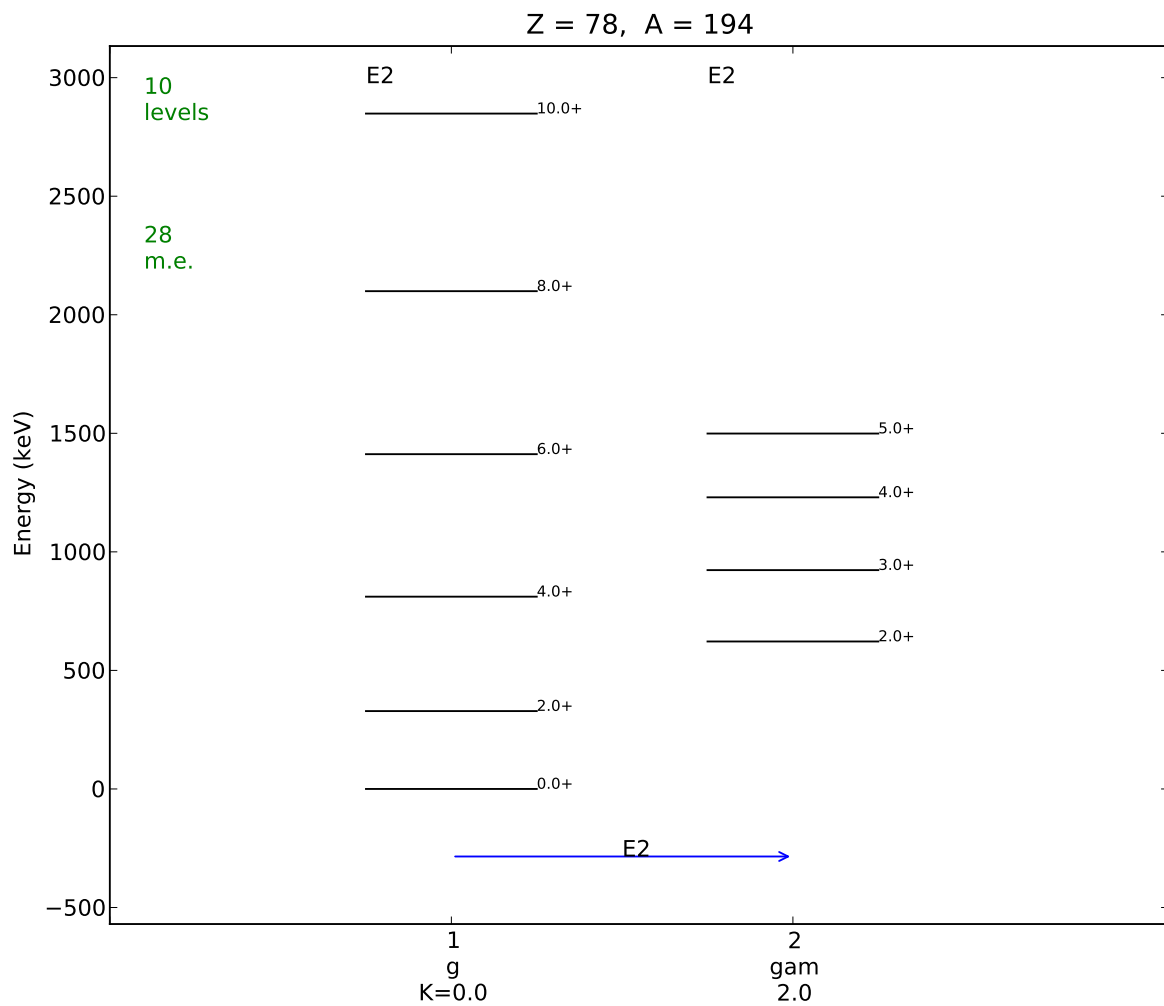
Figure 14.1: A partial level scheme of the nucleus to be investigated ( ^{194}\text{Pt} ) in the fit_demo_2011.tar files. The highest states in each band are “buffer” states, which are not observed in the experiment, but are required for accurate calculation of the yields of the lower levels. See section 7.14.
