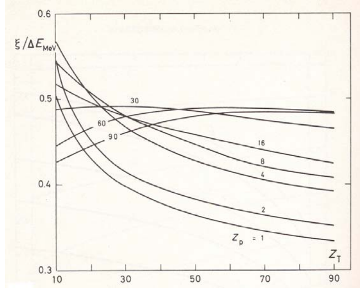
Figure 6.5: The ratio \xi_{NM}/\Delta E_{NM} versus Z_T and Z_P for Coulomb excitation at the maximum safe bombarding energy. Taken from [ALD75]
