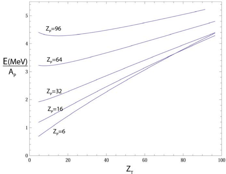
Figure 2.2: Maximum safe bombarding energy per nucleon according to equation 2.1 as a function of target Z_T value for selected projectile Z_P . The relation Z = 0.487 \frac{A}{1+0.00602A^{2/3}} was used to derive the corresponding A . [ALD75]
