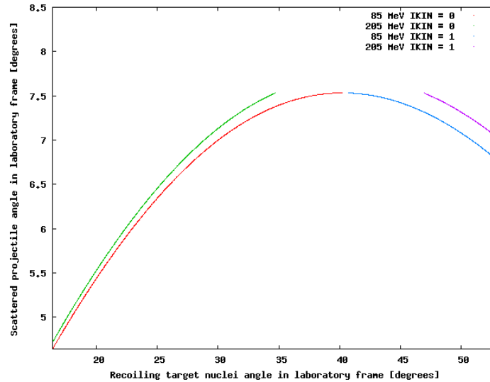
Figure 6.9: The angle of the scattered projectile in the laboratory frame for 194\text{MeV} ^{88}\text{Kr} beam on a ^{12}\text{C} target for bombarding energies of 85\text{MeV} and 205\text{MeV} .
