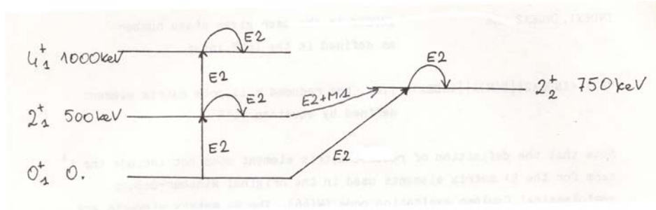
Figure 7.3: Model system having 4 states with E2 and M1 coupling. The 2_1^+ - 2_2^+ coupling is assumed to be of mixed M1 and E2 character.
