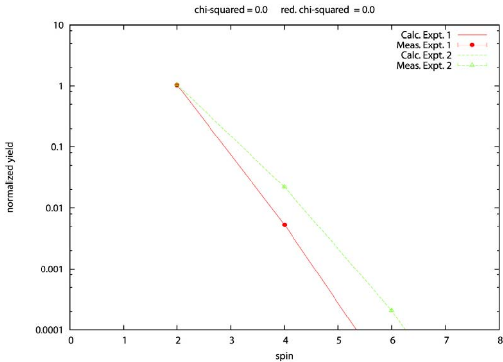
Figure 14.10: The measured (simulated) p - \gamma yield data and the predicted yields for the yrast states. Note that without introducing random scatter to the data results in extremely small value for the minimum value of \chi^2 .
