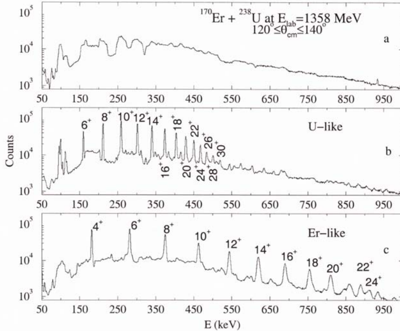
Figure 2.5: Typical \gamma -ray spectra for 1358\text{MeV} ^{238}\text{U} beam on a 0.5\text{mg}/\text{cm}^2 ^{170}\text{Er} target detected using Gammasphere in coincidence recoil ions detected by CHICO. (a) shows the raw coincident \gamma ray spectrum, (b) shows the coincident \gamma ray spectrum Doppler-corrected for U recoils, (c) shows the coincident \gamma ray spectrum Doppler-corrected for Er recoils. [WU00]
