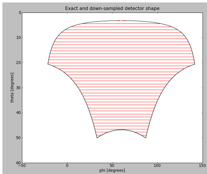
Figure 8.4: A rectilinear detector defined by the user in its plane and automatically transformed into the required \theta(\phi) sampling for GOSIA .
