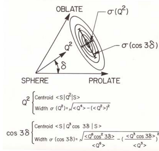
Figure 9.1: Distribution plot of the parameters Q^2 and \delta required to define the E2 properties in the intrinsic frame for a state S . All possible E2 moments are defined by the region Q \geq 0 and 0 \leq \delta \leq 60^\circ .
