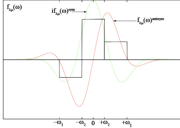
Figure 6.1: Actual and approximate Coulomb interaction strength functions. The fast approximation assumes that the antisymmetric component dominates in the ranges -\omega_1 \rightarrow -\omega_2 and +\omega_2 \rightarrow +\omega_1 while the symmetric component dominates in the range -\omega_2 \rightarrow +\omega_2 .
