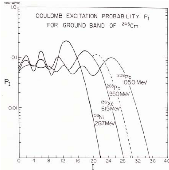
Figure 2.7: The calculated probability for Coulomb excitation of the ground band of ^{246}\text{Cm} by backscattered ions. The E2 matrix elements were assumed to be related by the spheroidal rotor relation. [CLI86]
