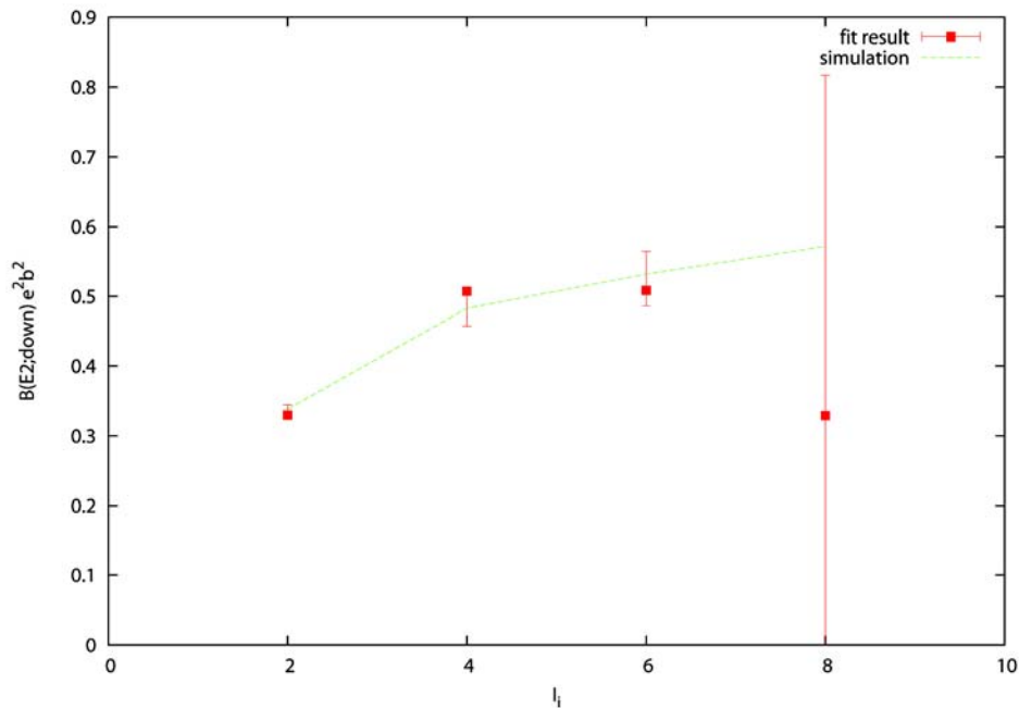
Figure 14.9: A example of a fit to simulated data for a ground-state band. The assumed matrix elements used to simulate the data are shown by the dashed green line while the red points plus errors correspond the the best fit matrix elements plus their correlated errors.
