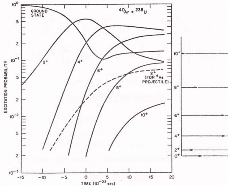
Figure 2.4: Semiclassical Coulomb excitation predictions of the time evolution for excitation of the ground-band in ^{238}\text{U} by backscattered 140\text{MeV} ^{40}\text{Ar} ions. [MCG69]
