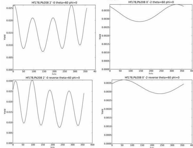
Figure 4.2: Upper row: Target excitation of ^{208}\text{Pb} by a 890\text{MeV} ^{178}\text{Hf} beam scattered at \theta_{proj} = 60^\circ . Lower row: Projectile excitation of a 890\text{MeV} ^{178}\text{Hf} beam scattered at \theta_{proj} = 60^\circ by a ^{208}\text{Pb} target. Left column: shows a 2^+ state at 1.175\text{MeV} decaying to the 0^+ ground state. Right column: shows a 1.0\text{MeV} 0^+ state decaying to the ground-band 2^+ state. The calculated yields are plotted versus \theta_\gamma which is measured with respect to the incident beam direction. The deorientation effect has been switched off.
