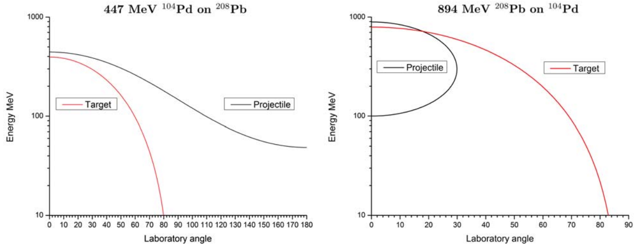
Figure 5.4: Recoil energies, in MeV , versus laboratory scattering angle. (Left) Scattering of 447MeV ^{104}\text{Pd} by ^{208}\text{Pb} for Q = -5.0MeV . (Right) Scattering of 894MeV ^{208}\text{Pb} on ^{104}\text{Pd} for Q = -5.0MeV .
