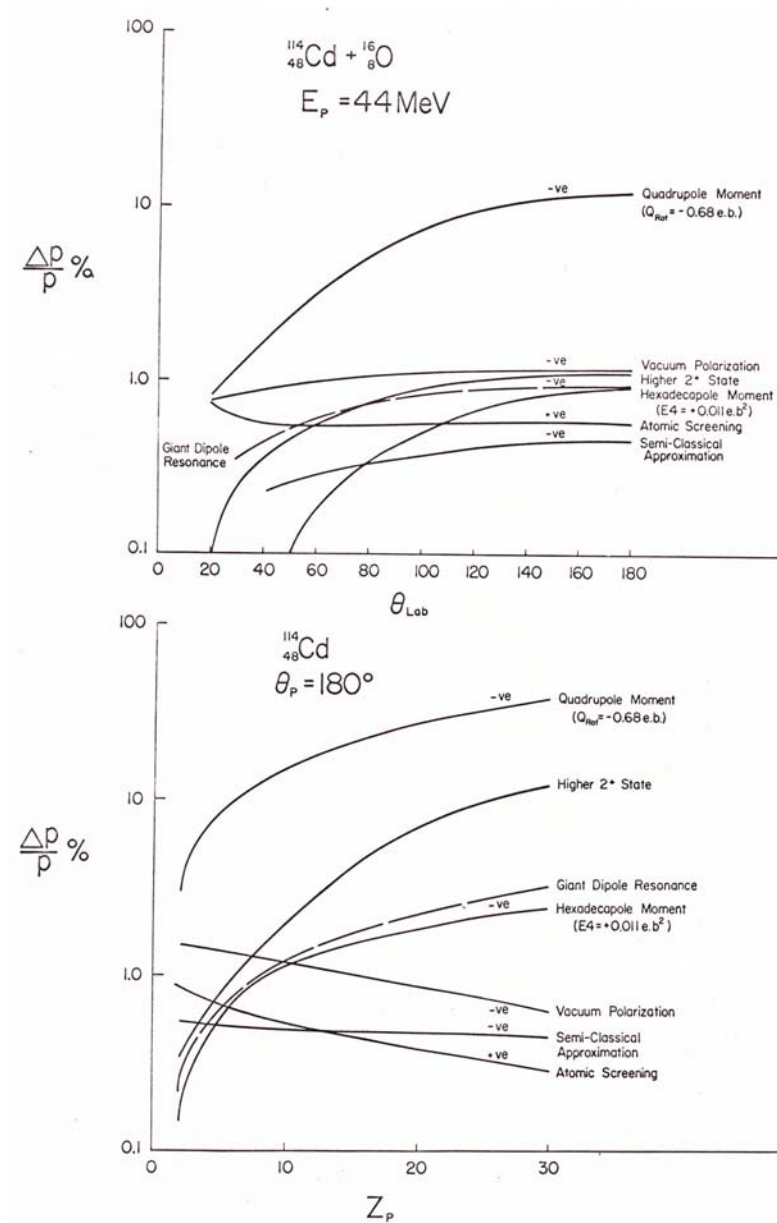
Figure 2.8: The importance of several effects on Coulomb excitation of the first excited 2_1^+ state in ^{114}\text{Cd} . The ordinate gives the % change in excited state excitation probability as a function of scattering angle (upper) and projectile Z_p (lower).
