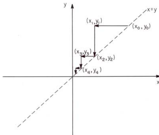
Figure 6.11: Simple steepest descent minimization of the function f(x, y) = x^2 + (x - y)^2
