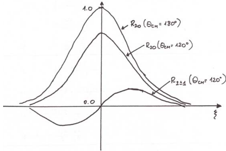
Figure 3.2: The orbital integrals R_{20} and R_{2\pm 1}
