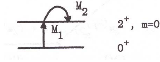
Figure 6.4: Reorientation effect for the two-level system.
