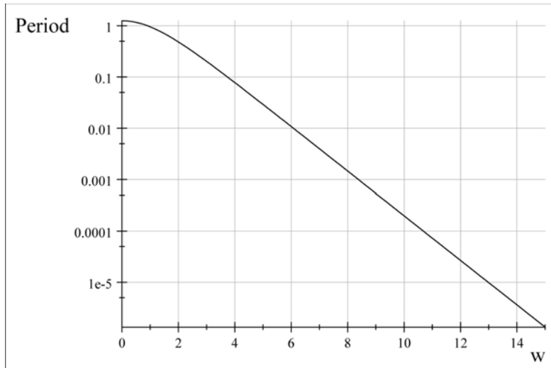
Figure 6.6: The period for one cycle of rotation of the phase factor and a function of \omega for the case of 300 MeV ^{136}\text{Xe} scattered at \theta_{cm} = 95^\circ exciting a 3 MeV 2^+ state in ^{180}\text{W} . This case corresponds to \xi = 2.13 , and \epsilon = 1.356 giving the product \xi\epsilon = 2.88 .
