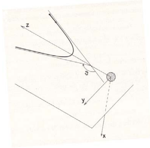
Figure 3.1: Coordinate system used to evaluate the Coulomb excitation amplitudes. The origin is chosen in the center of mass of the target nucleus. The x -axis is perpendicular to the plane of the orbit, the z -axis is along the symmetry axis of the incoming projectile orbit pointing towards the projectile, while the y -axis is chosen such that the y -component of the projectile velocity is positive. The scattering angle \theta of the projectile is shown. Note that Alder and Winther [ALD75] call this coordinate system B.
