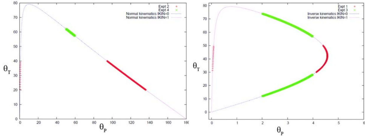
Figure 6.10: Left; Normal kinematics: Target recoil angle \theta_T versus projectile recoil angle \theta_P in the laboratory frame for 64\text{MeV} ^{12}\text{C} beam incident on a ^{148}\text{Sm} target. The red solid and hatched sections designate the two solutions for detection of the ^{148}\text{Sm} target recoils. The target recoil energies for the hatched solution are < 100\text{keV} which is below the recoil detector threshold. The solid green line designates detection of the ^{12}\text{C} projectile recoils. Right; Inverse kinematics: Target recoil angle \theta_T versus projectile recoil angle \theta_P in the laboratory frame for 356\text{MeV} ^{148}\text{Sm} ions on a ^{12}\text{C} target. The red solid and hatched sections designate the two kinematic solutions for detection of the ^{12}\text{C} target recoils. The target recoil energies for the hatched solution are < 100\text{keV} which is below the recoil detector threshold. The solid green line designates the two kinematic solutions for detection of the ^{148}\text{Sm} projectile recoils.
