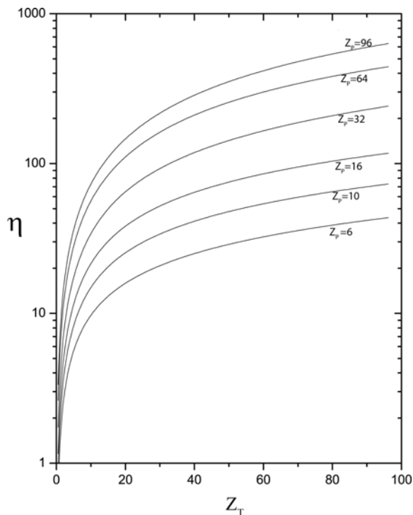
Figure 2.3: The Sommerfeld parameter \eta at the safe bombarding energy as a function of target Z_T for various projectile Z_P .
