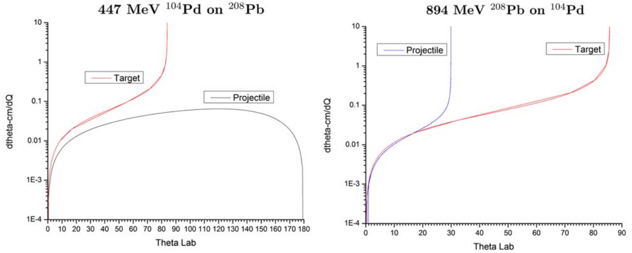
Figure 5.5: The magnitude of the derivatives \left| \frac{d\vartheta_{cm}^P}{dQ} \right| and \left| \frac{d\vartheta_{cm}^T}{dQ} \right| in degrees/MeV versus the laboratory scattering angle for the recoiling projectile and target with normal kinematics and inverse kinematics for inelastic scattering of 4.3 \text{ MeV/nucleon} ^{208}\text{Pb} by ^{104}\text{Pd} with Q = -5 \text{ MeV} . For normal kinematics the derivative goes to infinity at \theta_{lab}^T = 85.71^\circ . For inverse kinematics the derivatives go to infinity at the angle maxima \theta_{lab}^P = 29.907^\circ and \theta_{lab}^T = 85.71^\circ . The sign of the derivative \frac{d\vartheta_{cm}^P}{dQ} is negative for angles \vartheta_{cm}^P less than at the maximum of \theta_{lab}^P and positive for angles \vartheta_{cm}^P that are larger than at the maximum of \theta_{lab}^P . The sign of \frac{d\vartheta_{cm}^T}{dQ} is positive. Note that since \frac{d\vartheta_{cm}^P}{dQ} = -\frac{d\vartheta_{cm}^P}{d\Delta E} and \frac{d\vartheta_{cm}^T}{dQ} = -\frac{d\vartheta_{cm}^T}{d\Delta E} the signs for \frac{d\vartheta_{cm}^P}{d\Delta E} and \frac{d\vartheta_{cm}^T}{d\Delta E} are opposite to those given above. Note that the two-valued derivative curves overlap above and below the maximum recoil scattering angles in the laboratory frame.
