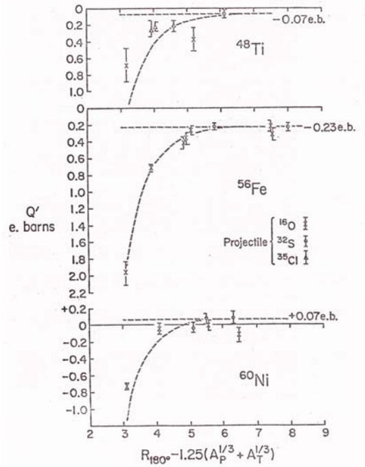
Figure 2.1: Effective values of the static quadrupole moment of the 2_1^+ states of ^{48}\text{Ti} , ^{56}\text{Fe} , and ^{60}\text{Ni} extracted from Coulomb excitation reorientation effect data plotted as a function of the classical separation distance between the nuclear surfaces for a head-on collision. [LES72]
