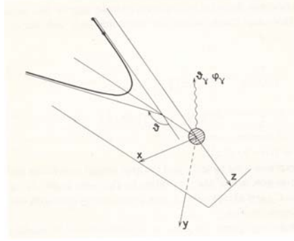
Figure 4.1: The coordinate system used to describe the \gamma -decay of a Coulomb-excited nucleus. The z -axis is chosen along the incoming beam direction, the x -axis is in the plane of the orbit such that the x -component of the velocity is positive. A \gamma -decay in the direction \theta_\gamma, \varphi_\gamma is indicated. Note that Alder and Winther [ALD75] call this coordinate system C .
