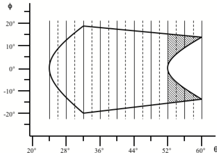
Figure 7.1: A rectangular particle detector has a non-azimuthally symmetric shape in the \theta, \phi space of projectile scattering angle. This shape must be defined by entering a number ( NFI ) of azimuthal angular ranges. In the hatched region, NFI = 2 ranges must be entered specifying the two active regions. The solid lines represent \theta meshpoints, while the dashed lines indicate \theta subdivisions. The rapid variation in active \phi range in the hatched region necessitates input of the active ranges of \Delta\phi at each subdivision specifying each of the two active detection regions shown hatched.
