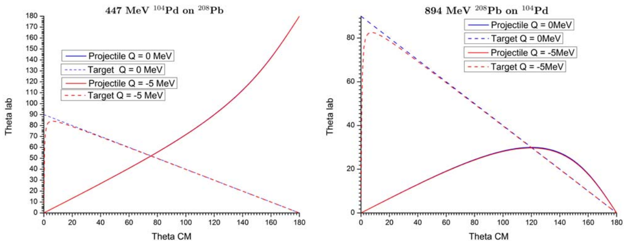
Figure 5.2: The kinematic correlation of the laboratory and centre-of-mass scattering angles of the recoiling projectile and target nuclei for scattering of 4.3\text{MeV/nucleon} ^{104}\text{Pd} on ^{208}\text{Pb} (left) and 4.3\text{MeV/nucleon} ^{208}\text{Pb} on ^{104}\text{Pd} (right). The projectile scattering angles are shown by solid lines while the recoiling target angles are shown by dashed lines. The blue curves correspond to elastic scattering Q = 0 , while the red curves correspond to inelastic scattering with Q = -5\text{MeV} .
