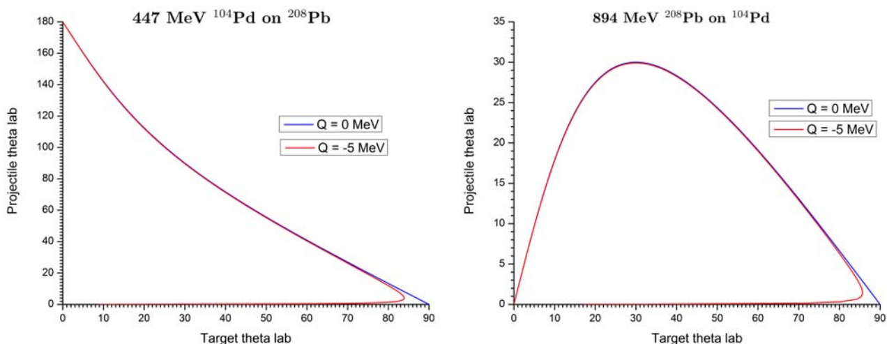
Figure 5.3: The kinematic correlation of the laboratory scattering angles for the recoiling projectile and target nuclei for scattering of a 4.3\text{MeV/nucleon} ^{104}\text{Pd} beam on ^{208}\text{Pb} (left), and a 4.3\text{MeV/nucleon} ^{208}\text{Pb} beam on ^{104}\text{Pd} (right). The blue curve is for elastic scattering, Q = 0 , and the red curve is for Q = -5\text{MeV} .
