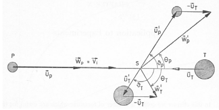
Figure 5.1: The velocities of the target and projectile before and after the collision. The velocities in the centre-of-mass system are denoted by \mathbf{u} and \mathbf{u}' respectively, while the velocities in the laboratory system are denoted by \mathbf{w} and \mathbf{w}' respectively. The indices P and T refer to projectile and target. Taken from [ALD75]
