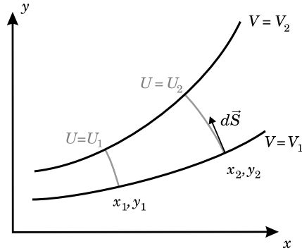
Figure 5.15: The charge on the lower plate between x_1, y_1 and x_2, y_2 is just \varepsilon_0(U_1 - U_2) .
