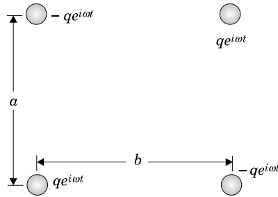
Figure 10.16: The electric quadrupole moment of problem 10-1.
