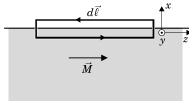
Figure 7.4: The Ampèrian loop lies in the x - z plane straddling the boundary.
