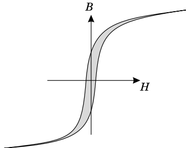
Figure 7.23: A good transformer core should have a thin hysteresis curve.
