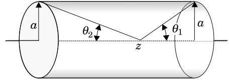
Figure 1.19: Geometry of the solenoid of question 21.
