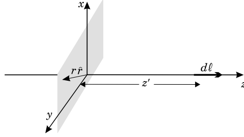
Figure 1.8: The current is assumed to run along the z axis, and we pick the observer in the x - y plane.
