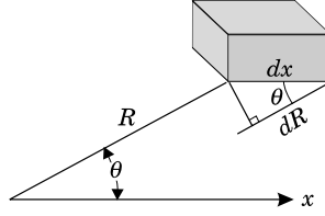
Figure 11.1: Fields from the far end of dx are emitted a time dt = dR/c earlier than those from the near end of the volume.
