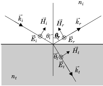
Figure 8.4: The electric vector of s -polarized light is perpendicular to the plane of incidence. The vectors illustrated refer to the fields at the vertex of the rays.
