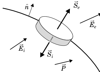
Figure 7.3: The Gaussian pillbox has ‘bottom’ surface \vec{S}_i with normal facing into the dielectric and ‘top’ surface \vec{S}_e with normal facing out.
