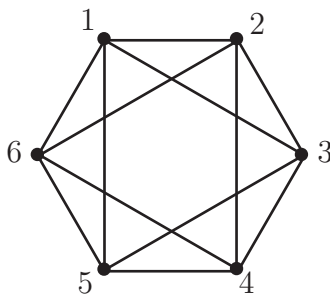
Figure 6.7: A graph on six vertices.
