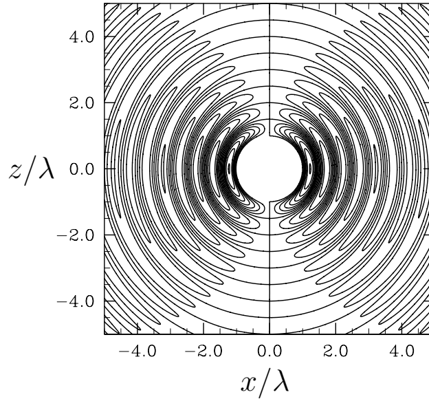
Figure 9.1: Equally spaced contours of the normalized poloidal electric field E_\theta/E_0 generated by a Hertzian dipole in the x - z plane at a fixed instant in time. Here, E_0 = \omega l I_0/4\pi\epsilon_0 c^2 .
