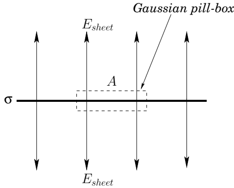
Figure 5.3: The electric field of a sheet charge.
