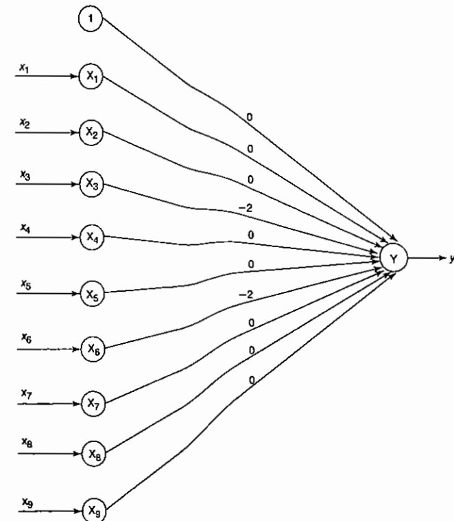
Figure 19 Hebb net of Figure 18.
