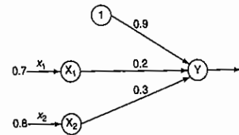
Figure 21 Neural net.
