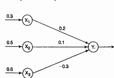
Figure 1 Neural net.
