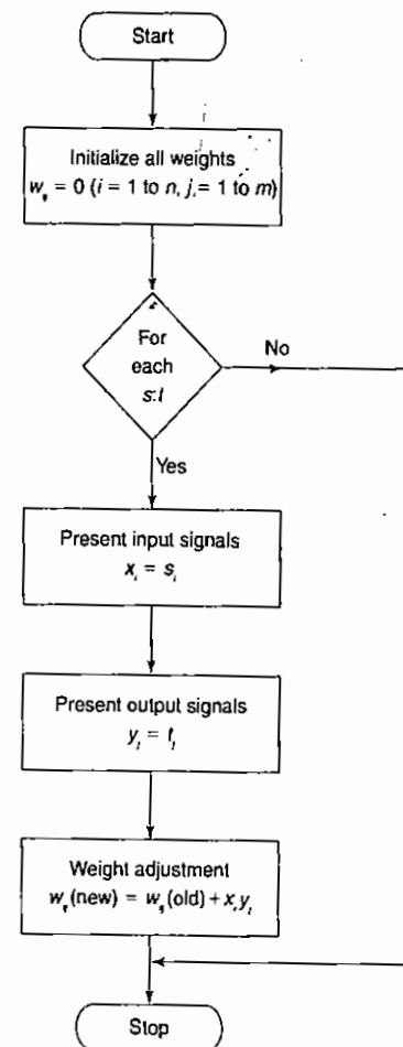
Figure 4-2 Flowchart for Hebb rule.
