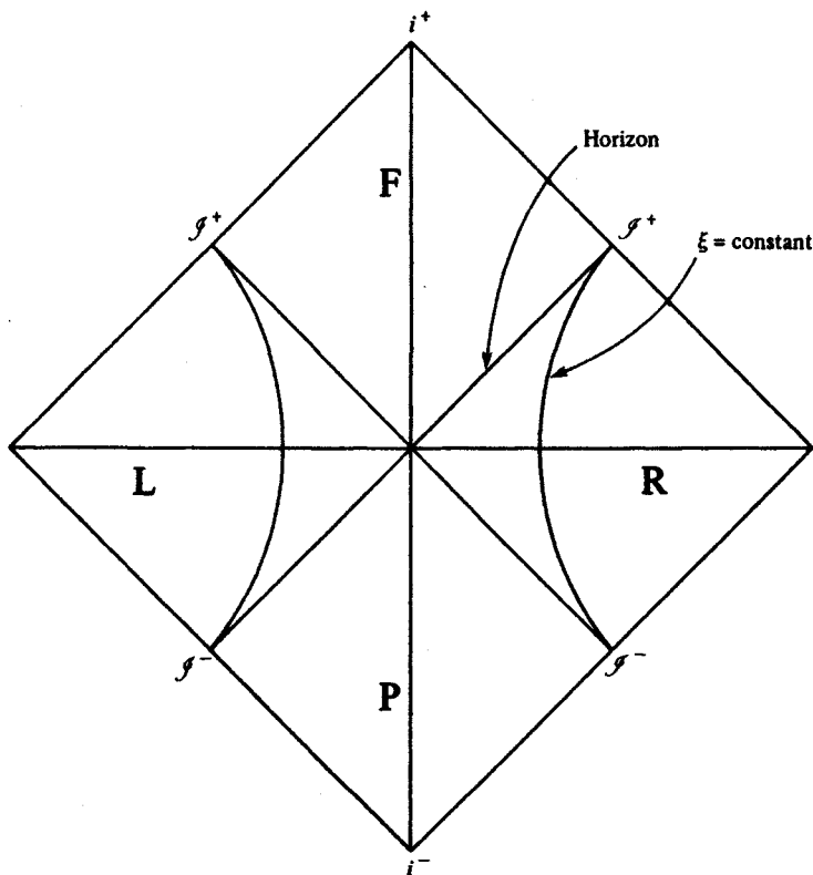
Fig. 14. Conformal diagram of Rindler system. The regions R, L, F and P are represented by diamond shaped regions. The timelike lines \xi = \text{constant} intersect \mathcal{I}^\pm , not i^\pm . Clearly, events in F cannot be witnessed in R, so the null ray \bar{u} = 0 ( u = \infty ) acts as an event horizon.
