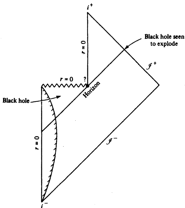
Fig. 27. Penrose diagram for an evaporating black hole. The lower portion of the diagram corresponds to fig. 25. However, when back-reaction is included, the hole evaporates, and the horizon intersects \mathcal{S}^+ at a finite time, after passing through a naked singularity (marked ?) Presumably the region above this is Minkowski space.
