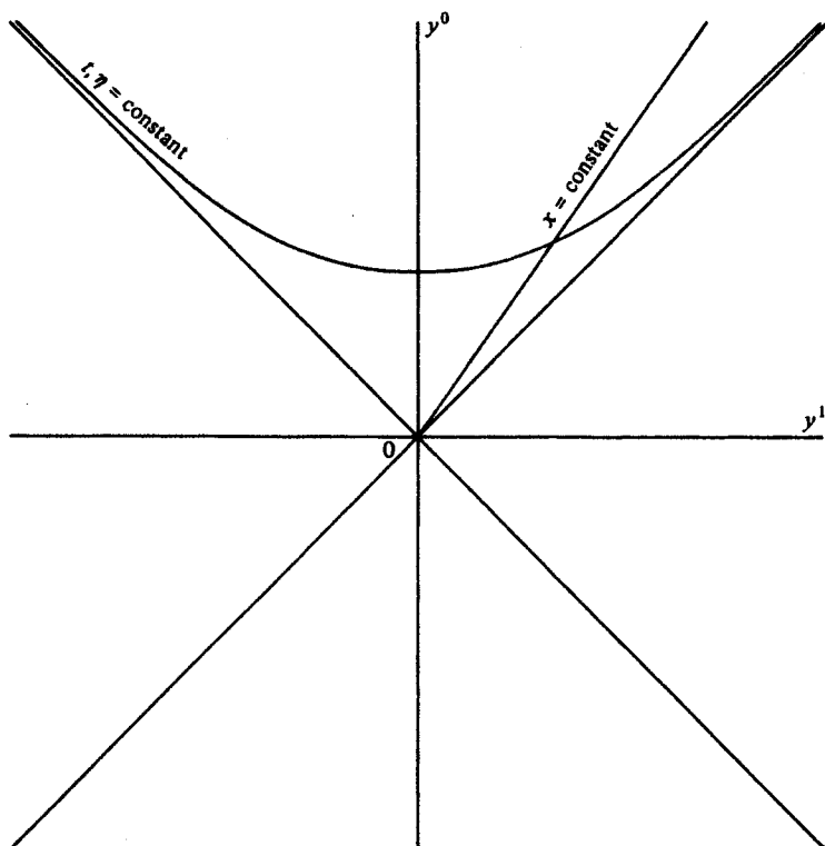
Fig. 15. Milne universe. The t, x coordinates cover the wedge of Minkowski space corresponding to region F in fig. 13. This region is therefore like the Rindler wedge on its side. The lines x = \text{constant} radiating from the origin represent the world lines of observers who perceive a universe expanding from a big bang origin at 0.
