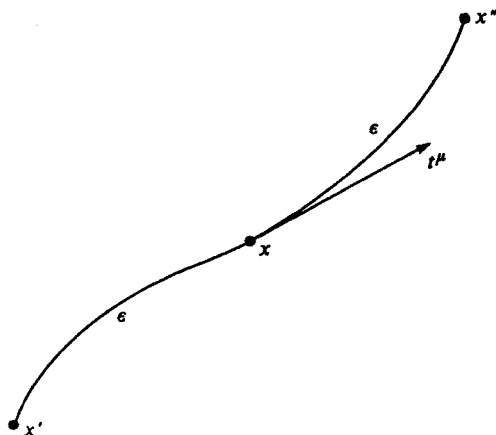
Fig. 22. The points x'' , x' lie along a non-null geodesic through x , parametrized by t^\mu , each a proper distance \epsilon from x .
