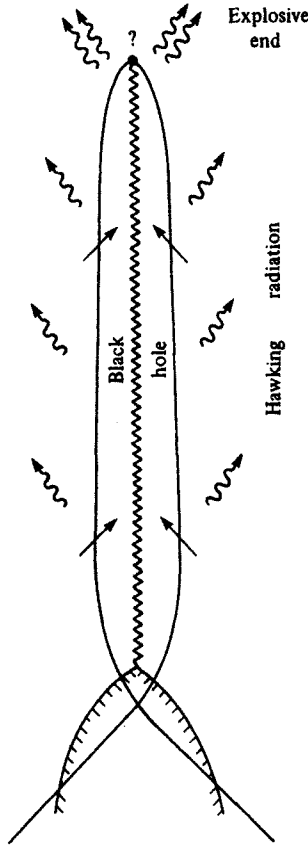
Fig. 26. Black hole evaporation. The lower portion of the diagram corresponds to fig. 24. Gradually the flux of negative energy crossing the horizon into the hole (straight arrows) causes the horizon area to shrink. The process escalates until the horizon collapses rapidly onto the singularity amid an explosive radiation of quanta.
