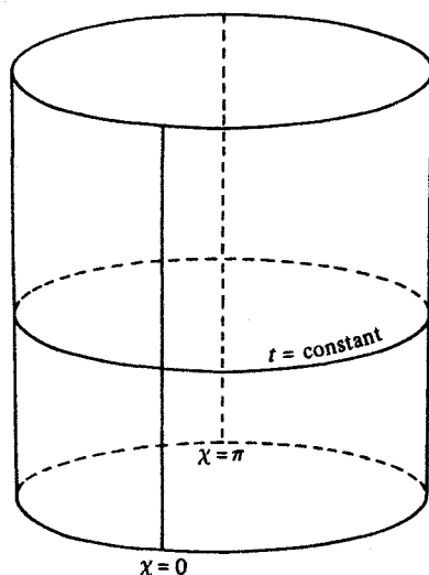
Fig. 19. Representation of the Einstein universe as a cylinder. The coordinates \theta and \phi are suppressed, t runs vertically from -\infty to +\infty and \chi runs around the cylinder.
