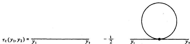
Fig. 29. Feynman diagram of the zeroth and first order contributions to the complete, connected propagator \tau_c(y_1, y_2) for \lambda\phi^4 theory.
