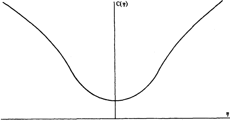
Fig. 8. The conformal scale factor C(\eta) = a^2 + b^2\eta^2 represents a universe that contracts to a minimum 'size' then re-expands symmetrically. At large \eta it behaves like a radiation-dominated Friedmann model.
