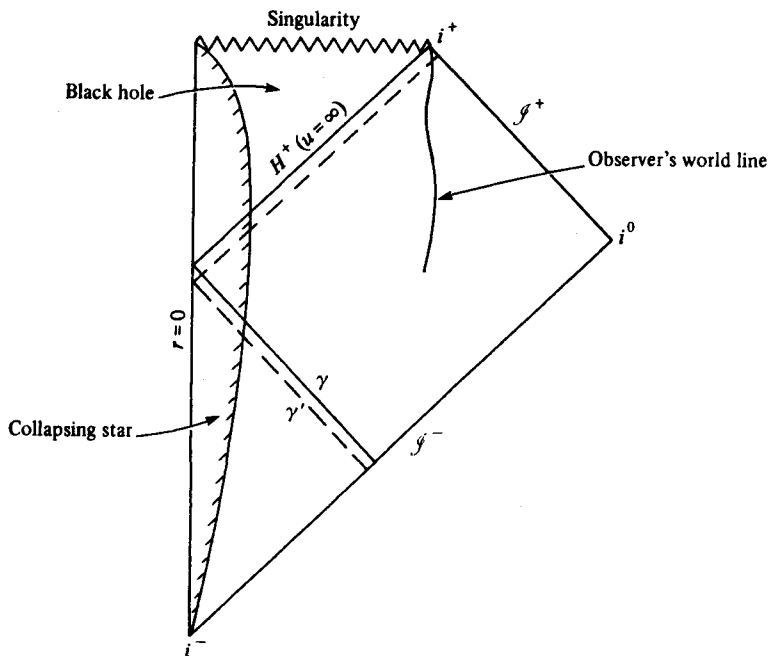
Fig. 25. Penrose diagram of a star that collapses to form a black hole. The exterior region is a fragment of fig. 6, including portions of regions I and III. The null ray \gamma passes through the centre of the star and emerges to form the event horizon ( u = \infty ), marked H^+ , as in fig. 24. A ray \gamma' (broken line) immediately prior to \gamma on \mathcal{S}^- reaches \mathcal{S}^+ at a finite value of u . Recalling the conformal compression of \mathcal{S} , one sees that the whole of the infinite future of the observer outside the hole corresponds to the narrow strip of null rays between \gamma and \gamma' , representing a brief duration on \mathcal{S}^- . Hence the infinity of equispaced late time null rays u = \text{constant} , when extended back through the star to \mathcal{S}^- , pile up next to \gamma inside this narrow strip.
