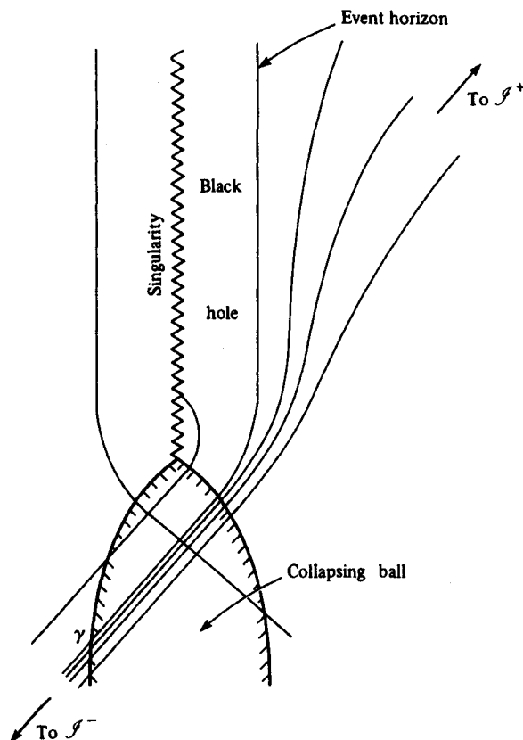
Fig. 24. As the ball collapses to a singularity, null rays converging on the ball's centre from \mathcal{J}^- are distorted. One such ray, labelled \gamma , forms the event horizon that marks the boundary between those rays that precede it and reach \mathcal{J}^+ , and later rays which are trapped by the black hole and drawn into the singularity. Rays which are equispaced along \mathcal{J}^+ at late times crowd up along \gamma on \mathcal{J}^- .
