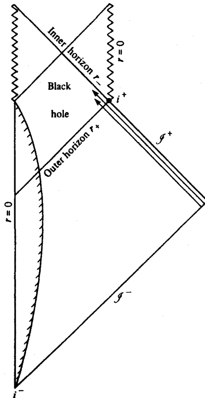
Fig. 28. Penrose diagram for a spherical star that collapses to form a charged, Reissner–Nordstrom, black hole. (Compare fig. 25. The manifold is drawn incomplete and can be extended vertically. This extension is irrelevant for the present discussion.) The singularity is timelike. Late time, infalling null rays from \mathcal{S}^- crowd up, blueshifted, along r_- .
