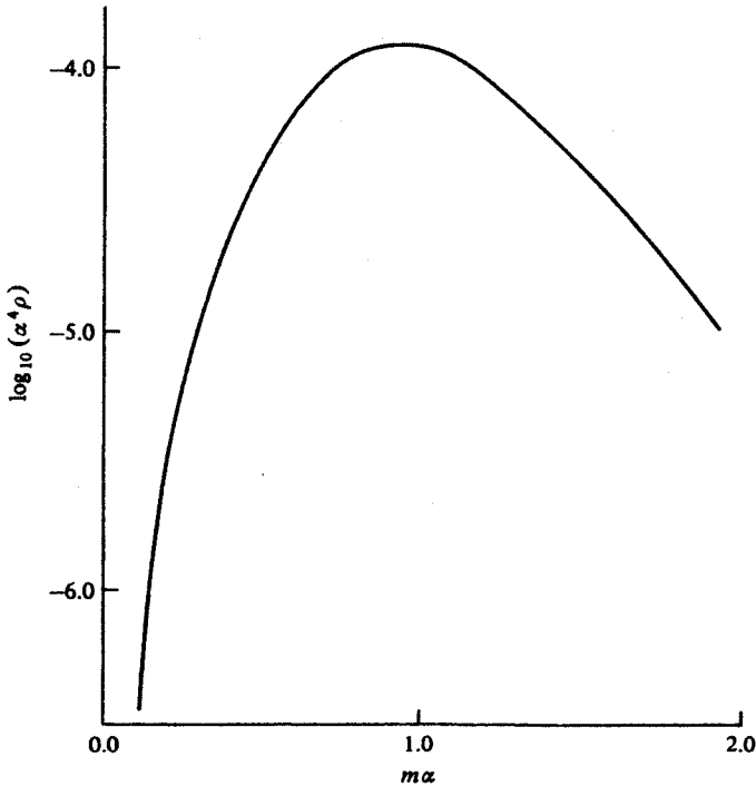
Fig. 23. The energy density of conformally coupled scalar particles created in a cosmological model with time dependence given by (7.80), as a function of particle mass.
