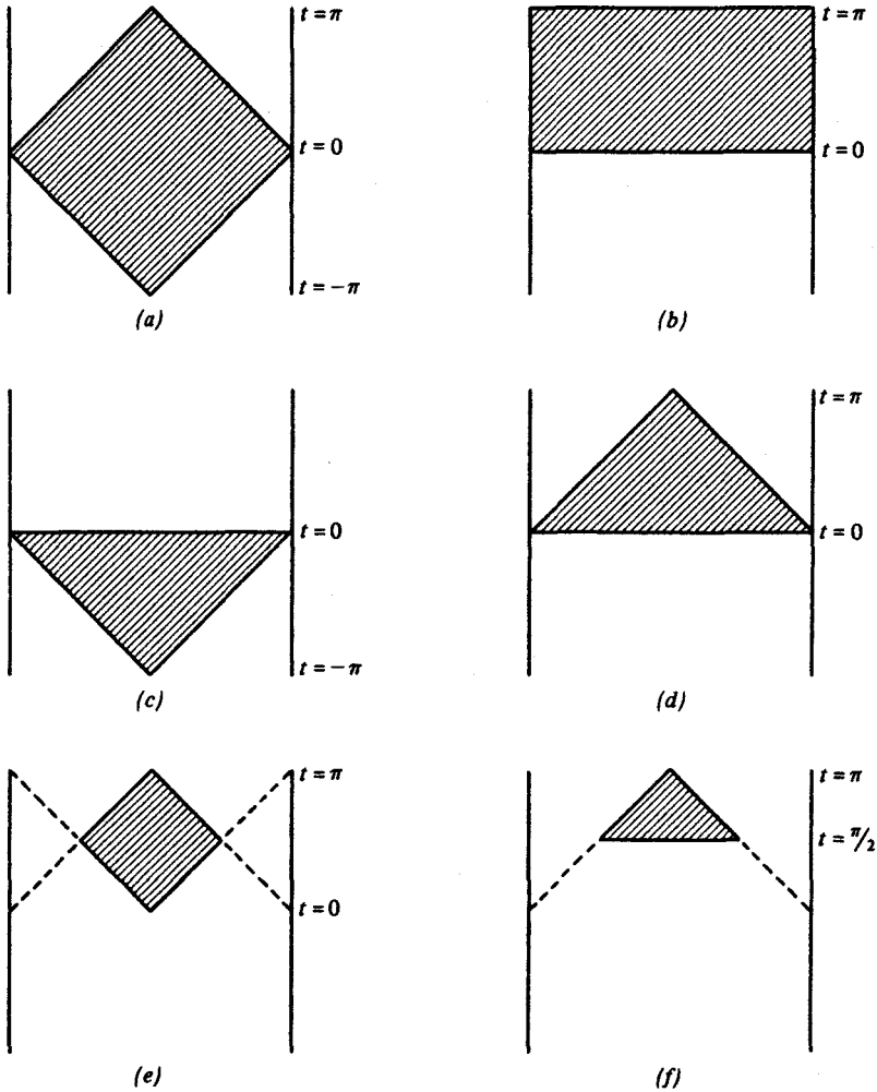
Fig. 20. The conformal images of various spacetimes in the Einstein cylinder. The coordinate t is the time coordinate in the Einstein cylinder (fig. 19). (a) Minkowski space, (b) de Sitter space and K = 1 Robertson-Walker spacetime, (c) steady-state universe, (d) K = 0 Robertson-Walker spacetime, (e) the Rindler wedge, static de Sitter space, the open Einstein universe and the Milne universe, (f) K = -1 Robertson-Walker spacetime. (After Candelas & Dowker 1979.)
