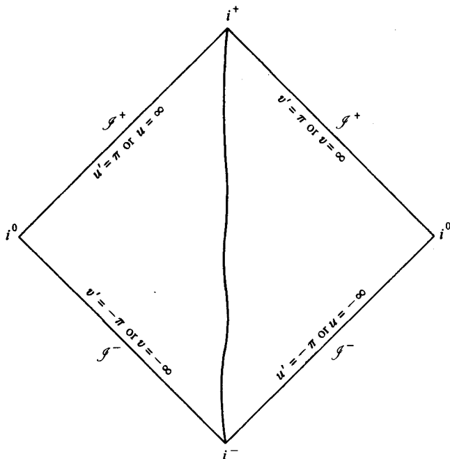
Fig. 4. Penrose conformal diagram of Minkowski space. The compact region -\pi \leq u', v' \leq \pi is conformal to the whole of Minkowski space ( -\infty \leq u, v \leq \infty ). Null rays u, v = \text{constant} remain at 45^\circ . The world line of an asymptotically timelike observer is shown.
