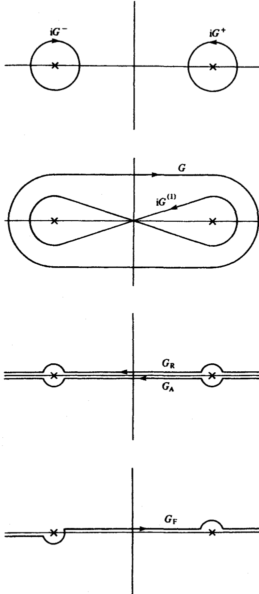
Fig. 3. The various Green functions are each associated with the above contours in the complex k^0 plane. The poles on the real axis at k^0 = \pm(|\mathbf{k}|^2 + m^2)^{1/2} are marked with crosses. The open contours should be envisaged as closed by infinite semicircles in the upper- or lower-half planes.
