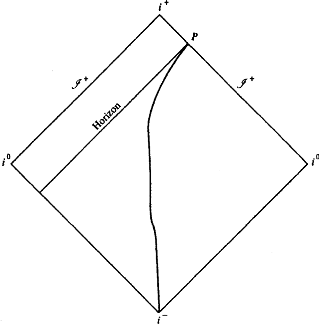
Fig. 5. The timelike world line represents an observer who accelerates continuously to the right, so that he asymptotically approaches the speed of light. This world line does not, therefore, reach i^+ , but intersects \mathscr{S}^+ at P . The backward null ray through P thus acts as an event horizon, because events above it can never be witnessed by the observer: all null rays from such events intersect \mathscr{S}^+ between P and i^+ .
