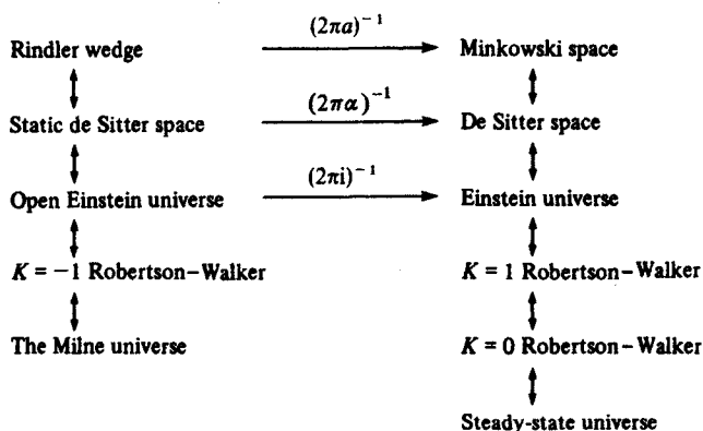
Fig. 21. Thermal and conformal relationships between various spacetimes. The vertical arrows indicate that the spacetimes are related by conformal transformations, while horizontal arrows represent relationship by thermalization at the temperature given. (After Candelas & Dowker 1979).
