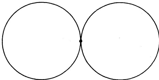
Fig. 30. Feynman diagram for the first order contribution to the vacuum-to-vacuum amplitude in \lambda\phi^4 theory.
