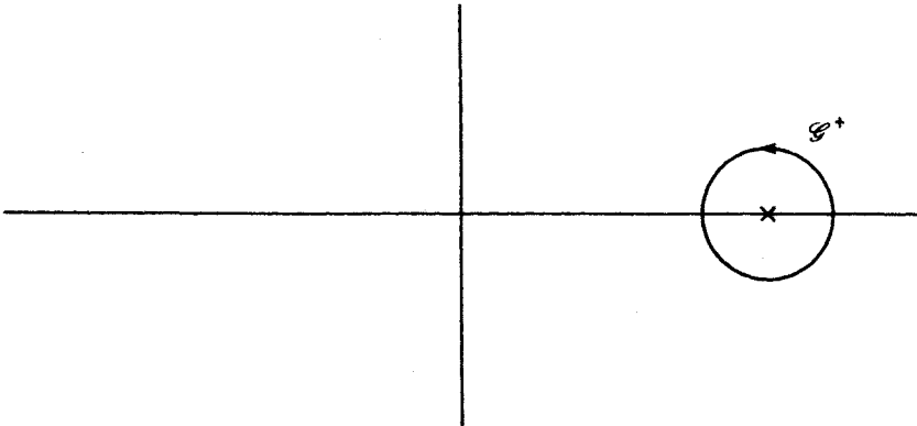
Fig. 9. The contour in the complex k^0 plane to be used in the evaluation of the integral giving \mathcal{G}^+ . The cross indicates the pole at k^0 = (|\mathbf{k}|^2 + m^2)^{1/2} .
