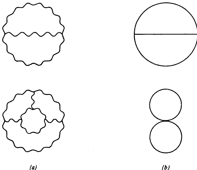
Fig. 2. (a) Higher order, multiple-loop graviton diagrams containing vertices. These represent contributions to the vacuum energy that diverge more strongly than that from fig. 1(b), and render quantum gravity non-renormalizable. (b) When non-gravitational interactions are introduced, multiple loops can also occur in the matter field diagrams.
