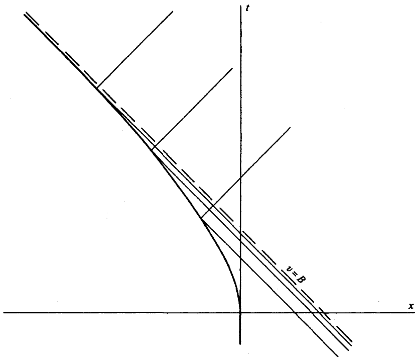
Fig. 12. The mirror trajectory, z(t) = -t - Ae^{-2\kappa t} + B , is asymptotic to the null ray, v = B . Late time surfaces of constant phase from \mathcal{I}^+ (equispaced null rays u = \text{constant} ) crowd up along v = B when reflected back off the mirror. Advanced (left-moving) rays later than v = B do not intersect the mirror at all. The radiation excited from the vacuum by this mirror trajectory has a thermal spectrum at late times.
