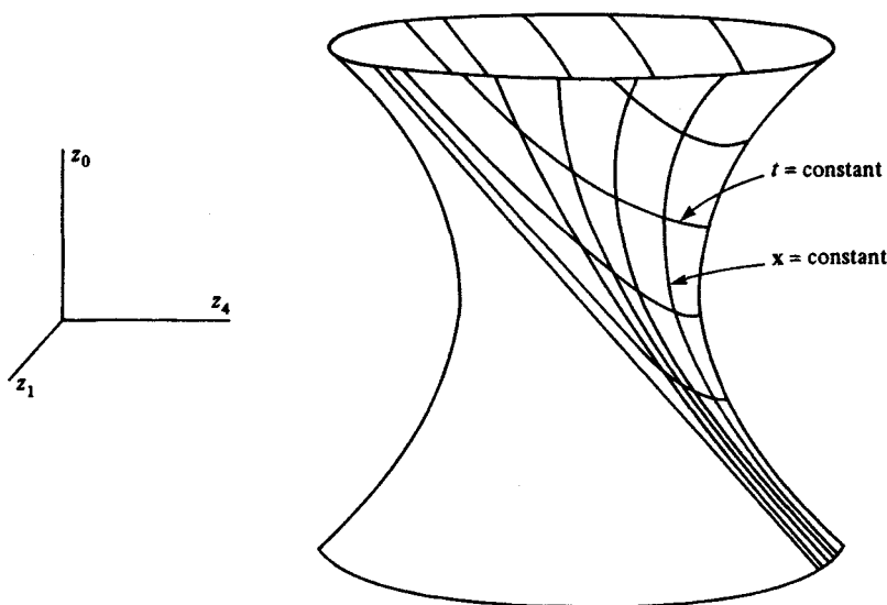
Fig. 16. De Sitter space represented as a hyperboloid embedded in five-dimensional flat spacetime (two dimensions are suppressed in the figure). The coordinates shown cover only half the space, called the steady-state universe, and are bounded by the null rays z_0 + z_4 = 0 ( t = -\infty ). The 3-spaces t = \text{constant} are flat, and expand with increasing t .
