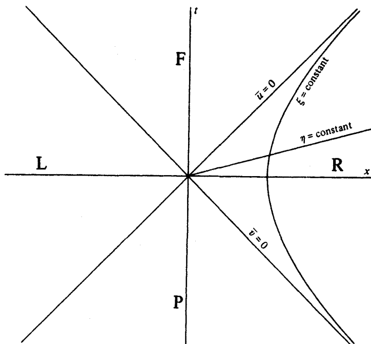
Fig. 13. Rindler coordinatization of Minkowski space. In R and L, time coordinates \eta = \text{constant} are straight lines through the origin, space coordinates \xi = \text{constant} are hyperbolae (corresponding to the world lines of uniformly accelerated observers) with null asymptotes \bar{u} = 0, \bar{v} = 0 , which act as event horizons. The four regions R, L, F and P must be covered by separate coordinate patches. Rindler coordinates are non-analytic across \bar{u} = 0 and \bar{v} = 0 .
