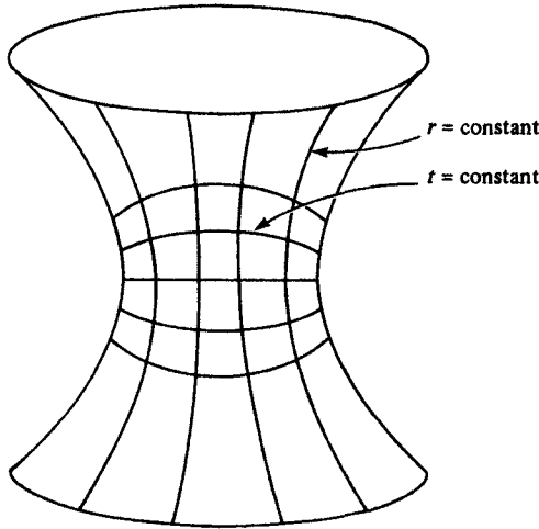
Fig. 18. De Sitter space as a static spacetime with metric (5.76).
