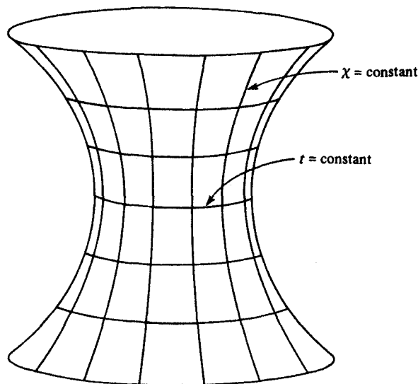
Fig. 17. De Sitter space represented as a contracting and re-expanding compact space with metric (5.65).
