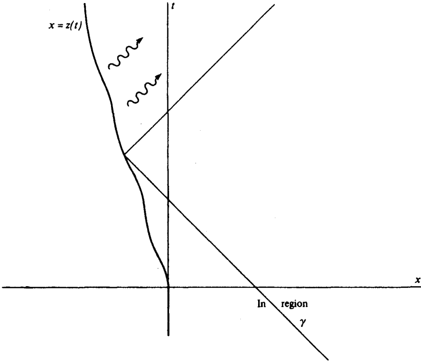
Fig. 11. Radiation by a moving mirror. The scalar field is constrained to vanish on the boundary x = z(t) . Null rays incoming from \mathcal{J}^- , such as \gamma , reflect from the mirror to \mathcal{J}^+ . Wave modes reflected after t = 0 suffer a Doppler shift in frequency due to the 'mirror' motion.
