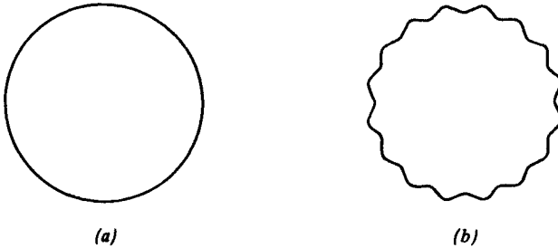
Fig. 1. Lowest order (one-loop) contribution to the vacuum energy from matter fields (a) and linearized gravitons (b) propagating in a prescribed background gravitational field.
