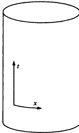
Fig. 10. Two-dimensional spacetime with compact spatial sections ( R^1 \times S^1 ). The circumference of the cylinder is L .
