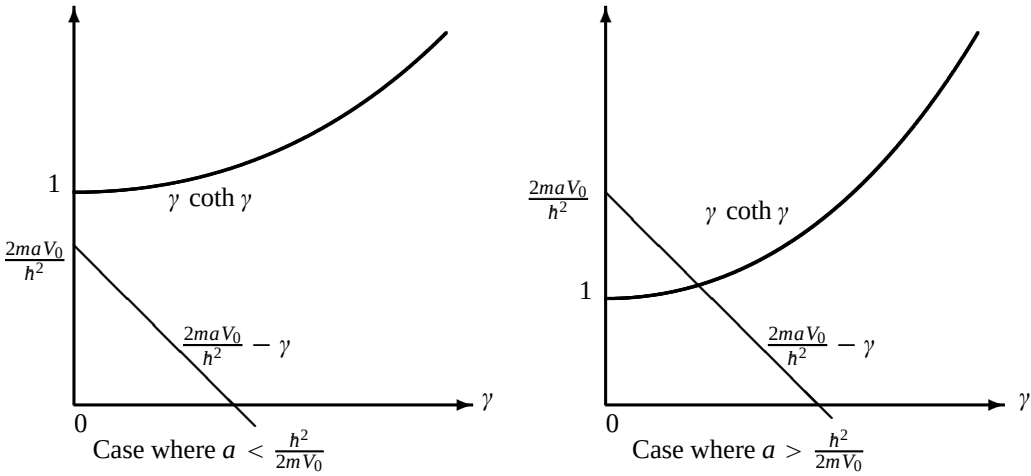
Figure 6.6 Graphical solutions of f(\gamma) = g(\gamma) , with \gamma = ka , f(\gamma) = \gamma \coth \gamma , and g(\gamma) = 2mV_0 a / \hbar^2 - \gamma . If a < \hbar^2 / (2mV_0) there is no bound state. If a > \hbar^2 / (2mV_0) there is one bound state.
