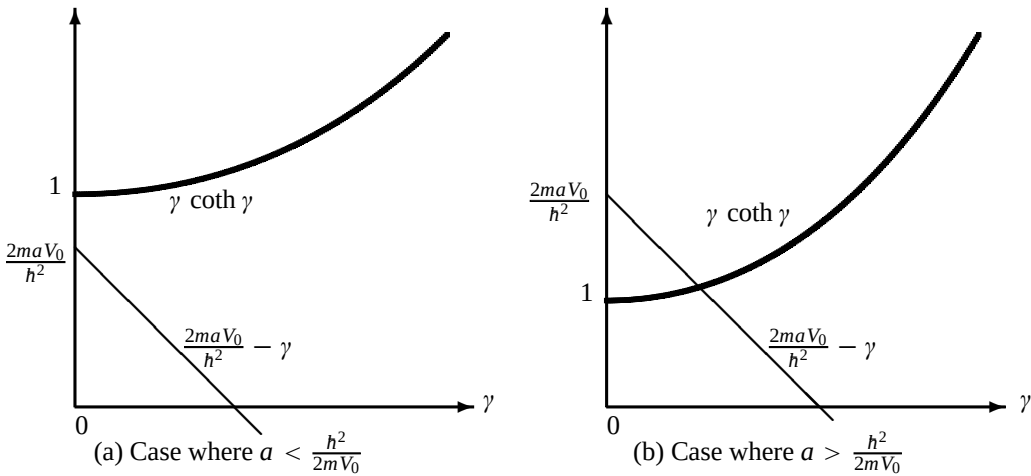
Figure 4.15 Graphical solutions of h(\gamma) = u(\gamma) , with \gamma = ka , h(\gamma) = \gamma \coth \gamma , and u(\gamma) = 2mV_0 a / h^2 - \gamma . If a < 2mV_0 / h^2 there is no bound state. If a > 2mV_0 / h^2 there is one bound state.
