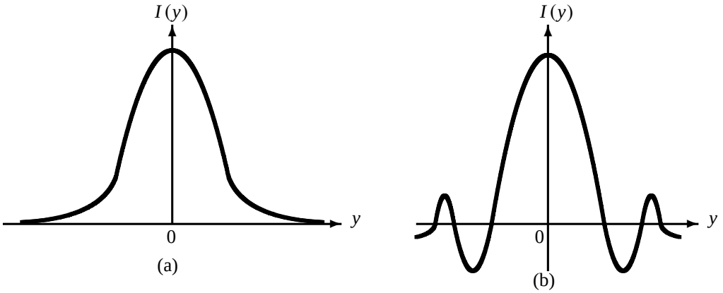
Figure 1.17 Shape of the total intensity generated in a double slit experiment when both slits are open and (a) a light source is used to observe the electrons' motion, I(y) = 2/\pi(1+y^2) , and no interference is registered; (b) no light source is used, I(y) = 4/[\pi(1+y^2)] \cos^2(\pi y/2) , and an interference pattern occurs.
