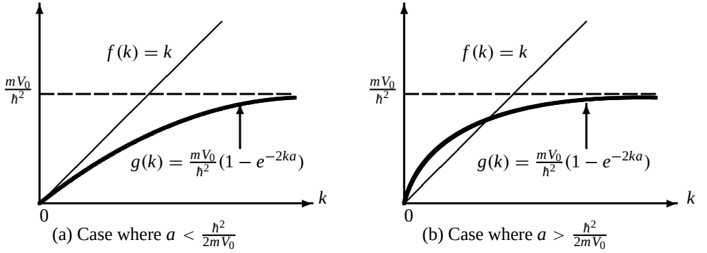
Figure 4.14 Graphical solutions of f(k) = g(k) or k = (mV_0/h^2)(1 - e^{-2ka}) . If the slope of g(k) is smaller than 1, i.e., a < h^2/(2mV_0) , no bound state will exist, but if the slope of g(k) is greater than 1, i.e., a > h^2/(2mV_0) , there will be only one bound state.
