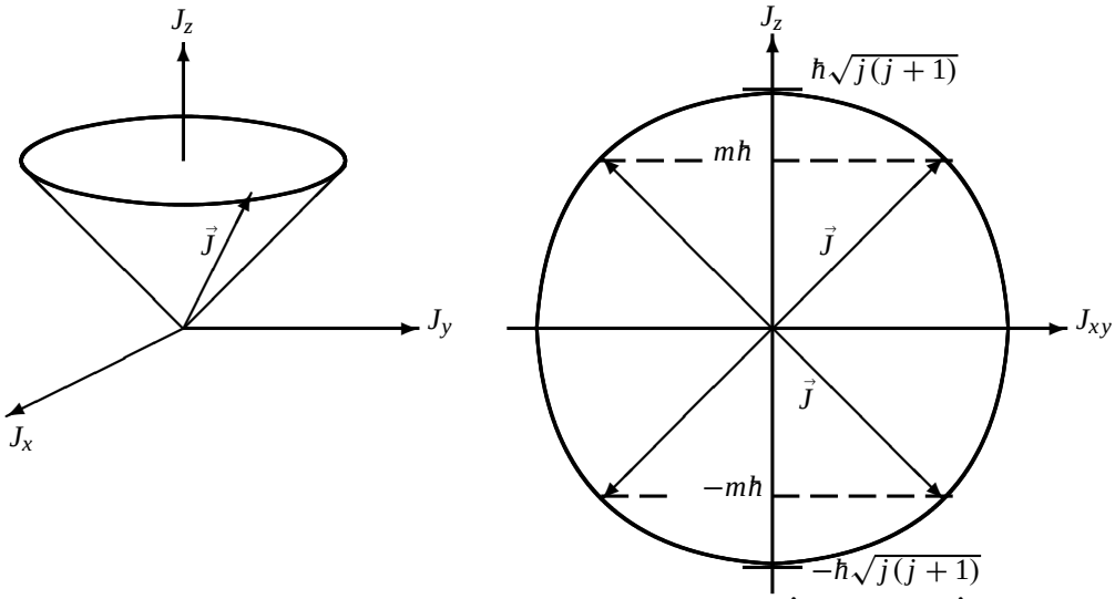
Figure 5.1 Geometrical representation of the angular momentum \hat{\vec{J}} : the vector \hat{\vec{J}} rotates along the surface of a cone about its axis; the cone's height is equal to mh , the projection of \hat{\vec{J}} on the cone's axis. The tip of \hat{\vec{J}} lies, within the J_z J_{xy} plane, on a circle of radius \hbar\sqrt{j(j+1)} .
