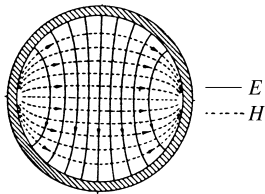
Figure 7.7 Field configuration for the \text{TE}_{11} (dominant) mode in a circular waveguide. (Adapted from Ref. 2 with permission.)
