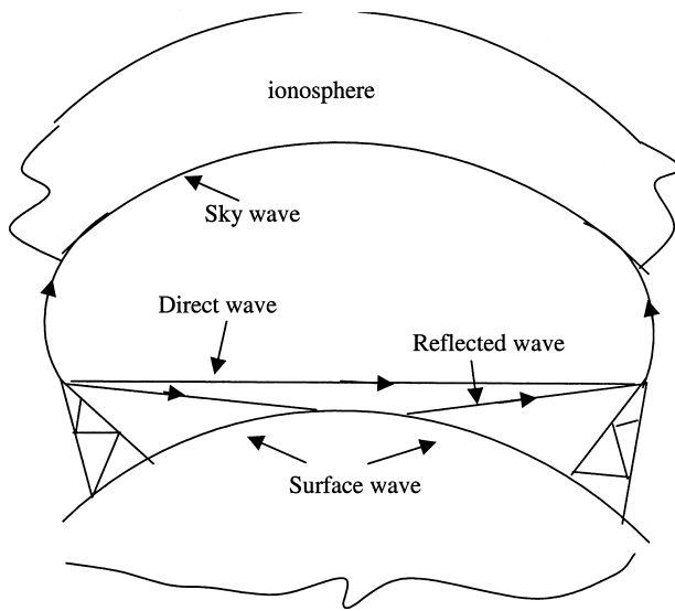
Figure 5.6 Modes of wave propagation.
