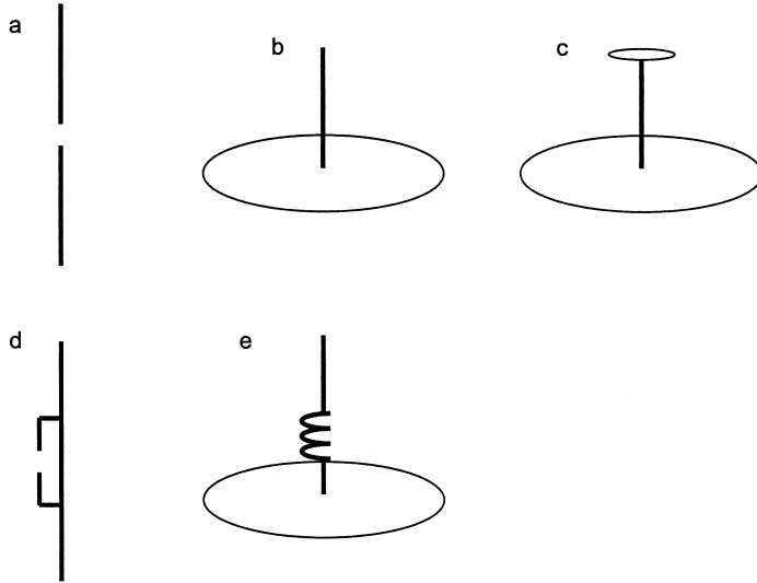
Figure 8.9 Variations on a straight wire antenna. (a) center-fed dipole antenna, (b) end-fed monopole antenna above a ground plane, (c) capacitive loaded monopole antennas, (d) T-feed dipole antennas, and (e) coil-loaded monopole antenna.
