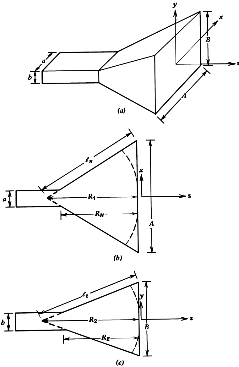
Figure 9.32 Pyramidal horn antenna: (a) perspective view, (b) H-plane ( xz plane) cross section, and (c) E-plane ( yz plane) cross section.
