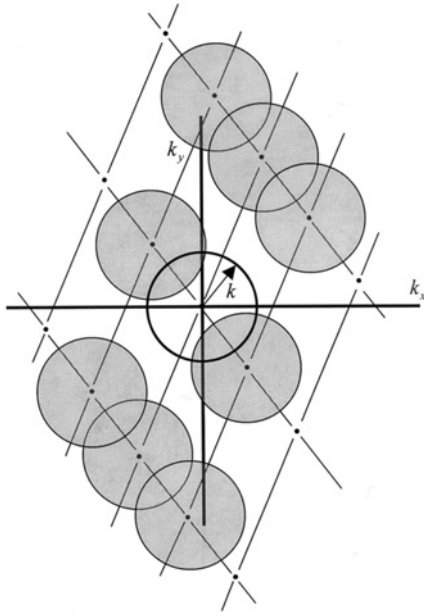
Figure 9.38 Grating-lobe lattice. The circle centers correspond to grating-lobe positions when the main beam is at broadside. As the array main beam is scanned within the visible region (the central unshaded circle), the grating lobes scan within the shaded circles. Grating-lobes enter the visible region when the main beam is scanned to a point in a shaded region overlapping the visible region circle.
