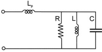
Figure 9.7 CAD model for the input impedance of a coaxial probe-fed microstrip antenna, operating near the resonance frequency.
