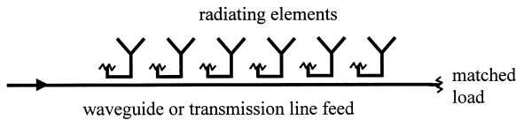
Figure 9.44 Series feed array using directional couplers.
