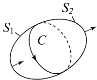
Figure 3.2 Two surfaces, S_1 and S_2 , defined by a common contour C , form a closed surface to which the law of conservation of magnetic flux applies—the magnetic flux through them is the same. The direction chosen for the loop determines the normal vector directions for S_1 and S_2 according to the right-hand rule.
