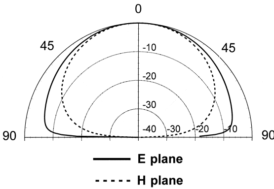
Figure 9.4 The radiation patterns for a rectangular patch antenna on an infinite substrate of permittivity \epsilon_r = 2.2 and thickness h/\lambda_0 = 0.02 . The patch is resonant with W/L = 1.5 . The E-plane ( xz plane) and H-plane ( yz plane) patterns are shown.
