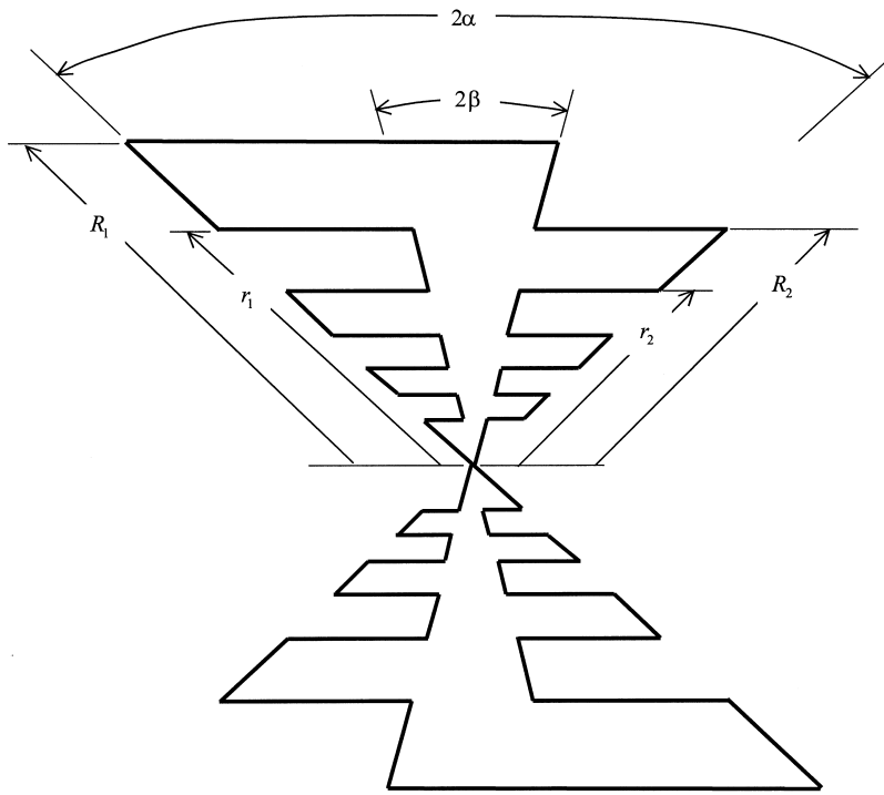
Figure 9.18 Planar trapezoidal-tooth log-periodic antenna.
