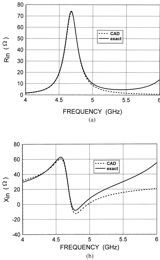
Figure 9.8 Input impedance versus frequency for a rectangular coaxial probe-fed patch antenna. The results from the CAD model in Fig. 9.7 are compared with those obtained by a cavity-model analysis: (a) input resistance and (b) input reactance. L = 2.0 cm and W/L = 1.5 . The feed probe is located at x_0 = L/4 , y_0 = W/2 and has a radius of 0.05 cm. The substrate has a permittivity of \epsilon_r = 2.2 and a thickness of 0.1524 cm.
