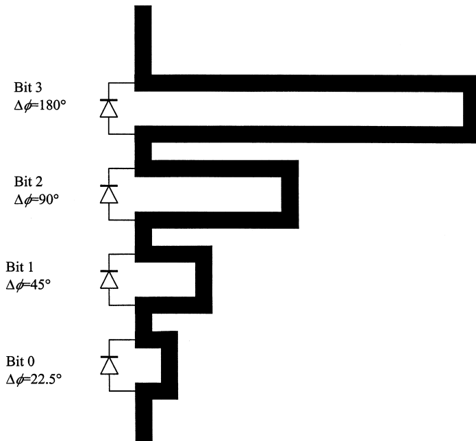
Figure 8.15 Serpentine digital phase shifter electrically controlled by p.i.n. diodes that short-circuit the microstrip line with an applied voltage.
