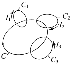
Figure 3.3 Three current loops and the illustration of Ampere's law. The line integral of \mathbf{B} along C in the case shown equals I_1 - I_2 - I_3 .
