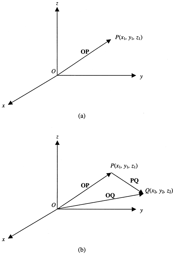
Figure C.3 (a) The position vector \mathbf{OP} extends from the origin O to the point P . (b) The distance vector \mathbf{PQ} extends from P to Q .
