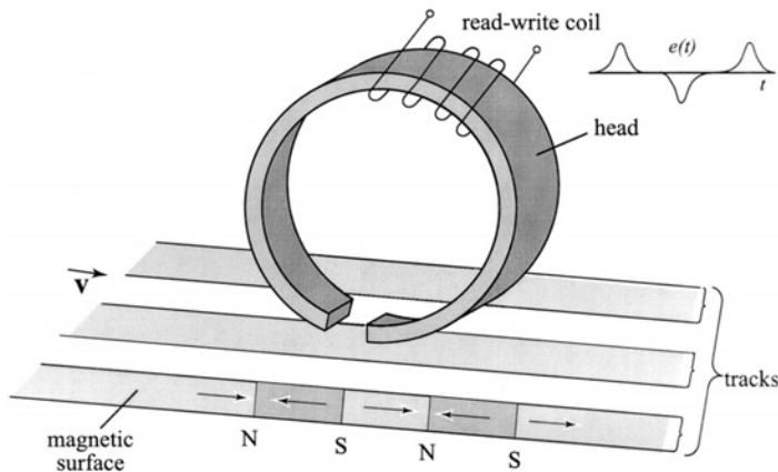
Figure 4.13 A hard disk magnetized through the write process induces a emf in the read process: when the recorded magnetic domains change from south to north pole or vice versa, a voltage pulse proportional to the remanent magnetic flux density is produced. The pulse can be negative or positive.
