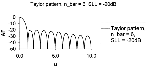
Figure 9.40 Pattern of a continuous Taylor aperture distribution: \bar{n} = 6 , \text{SLL} = -20\text{ dB} .
