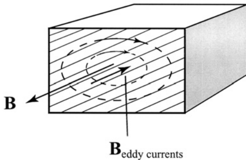
Figure 4.5 Eddy currents in a piece of ferromagnetic core. Note that the total \mathbf{B} field in the core is reduced due to the opposite field created by eddy currents.
