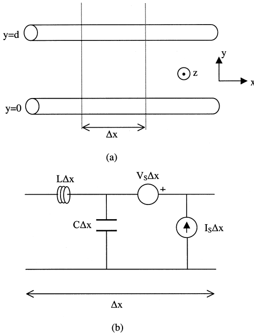
Figure 10.15 Coupling of an external field onto a two-wire line (a) and circuit model (b).
