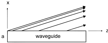
Figure 9.24 An illustration of the near-field behavior of a leaky wave on a guiding structure that begins at z=0 (illustrated for the leaky-wave antenna of Fig. 9.22). The rays indicate the direction of power flow in the leaky-wave field, and the closeness of the rays indicates the field amplitude. This figure illustrates the exponential growth of the leaky-wave field in the x direction out to the leakage boundary.
