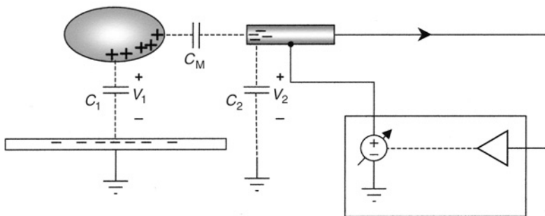
Figure 2.18 Using a noncontacting voltmeter to measure a charged, electrically isolated conductor.
