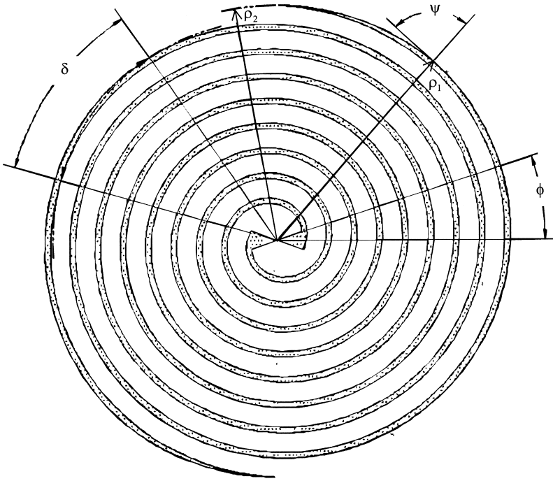
Figure 9.16 Planar two-arm Archimedean spiral antenna.
