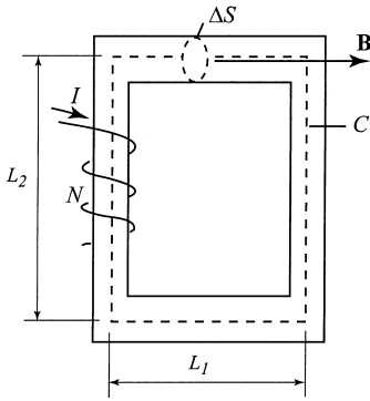
Figure 3.9 A thin magnetic circuit. L_1 and L_2 are lengths of the core sides along contour C through the center of the magnetic core of cross-section \Delta S .
