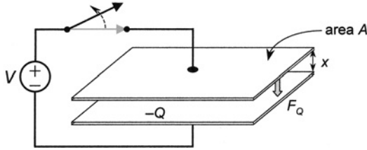
Figure 2.7 Parallel electrodes are energized by a voltage source that is subsequently disconnected. Fixed charges \pm Q remain on the electrodes.
