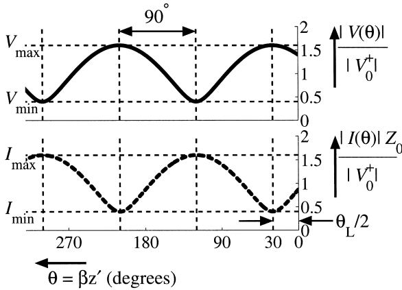
Figure 6.17 Voltage and current standing-wave patterns for a lossless transmission line terminated in a complex load impedance with \Gamma_L = 0.6 e^{j60^\circ} .
