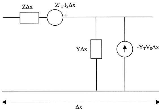
Figure 10.12 Model of a cable segment including transfer impedance and admittance.
