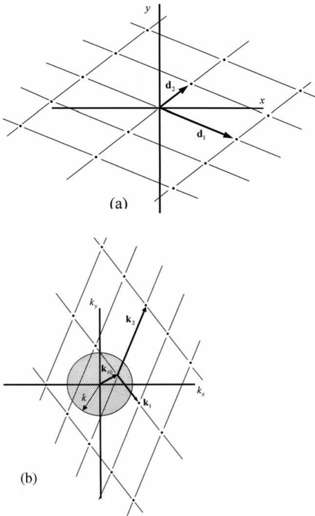
Figure 9.36 (a) The element lattice is defined by the lattice vectors \mathbf{d}_1 and \mathbf{d}_2 . (b) The grating lobe lattice is shown translated by \mathbf{k}_{r0} , the phasing needed to scan the array beam within the circle representing the visible region. Lattice vectors \mathbf{d}_1 and \mathbf{d}_2 are usually chosen such that no grating lobes appear within the visible region as \mathbf{k}_{r0} varies over the desired scan range.
