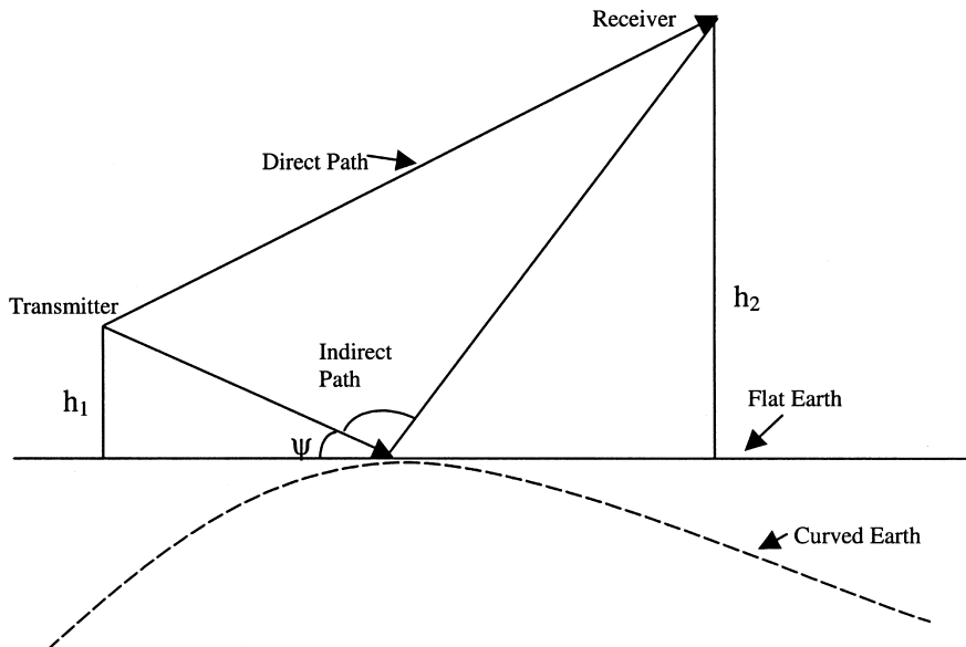
Figure 5.7 Multipath geometry.
