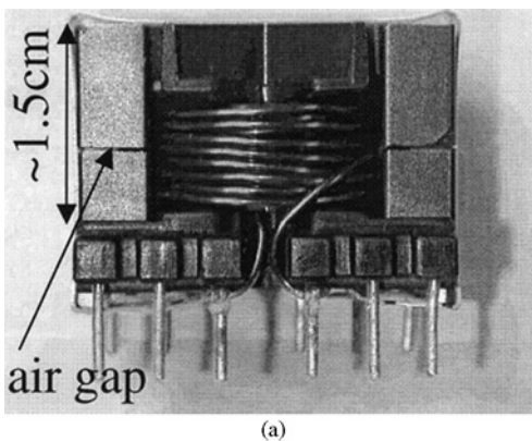
Figure 4.17 (a) A low-frequency inductor, with L \approx 1 mH, wound on a core with an air gap, (c) an inductor with a permalloy core with L \approx 0.1 mH, (c) a printed inductor surrounded by a ferromagnetic core with L \approx 10 \mu H, (d) small higher frequency inductors with L \approx 1 \mu H, (e) a chip inductor for surface-mount circuits up to a few hundred MHz with L \approx 0.1 \mu H, and (f) a micromachined spiral inductor with L \approx 10 –20 nH and a cutoff frequency of 30 GHz ( Q > 50 ).
