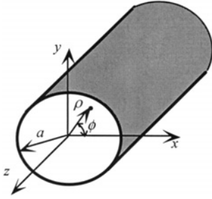
Figure 7.6 A circular waveguide.
