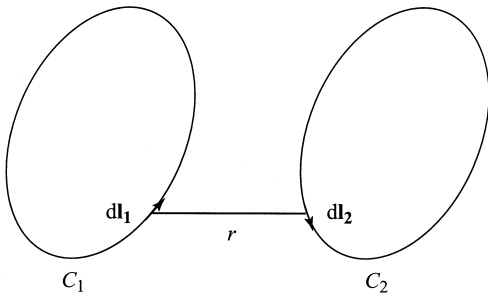
Figure 4.20 Two loops made out of thin wire.
