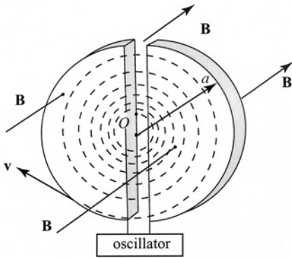
Figure 3.11 Sketch of a cyclotron used in scientific research to accelerate charged particles by means of electric and magnetic fields.
