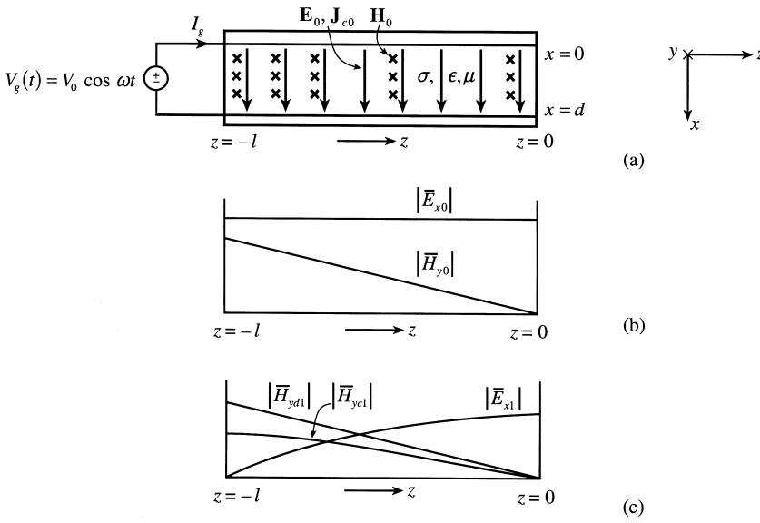
Figure 1.19 (a) Zero-order fields for the parallel-plate structure of Fig. 1.15. (b) Variations of amplitudes of the zero-order fields along the structure. (c) Variations of amplitudes of the first-order fields along the structure.
