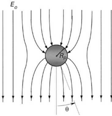
Figure 2.8 Conducting sphere distorts an otherwise uniform electric field. The field components are given by Eq. (2.32). If the source of the field produces ions, the latter will follow the field lines to the particle surface.
