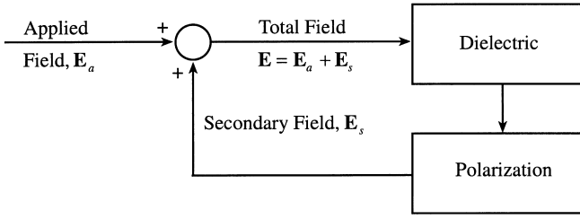
Figure 1.3 Illustrates the effect of polarization in a dielectric material.
