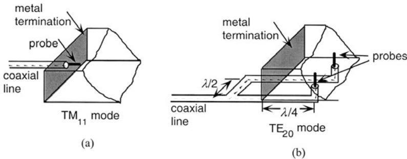
Figure 7.11 Coaxial-to-rectangular transitions that excite the TM_{11} and TE_{20} modes.
