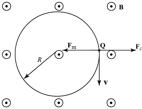
Figure 3.10 Charged particle in a uniform magnetic field.
