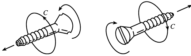
Figure 1.9 Right-hand-screw-rule convention.
