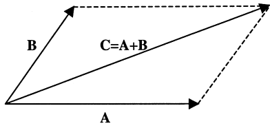
Figure C.2 Vector addition via the parallelogram rule.
