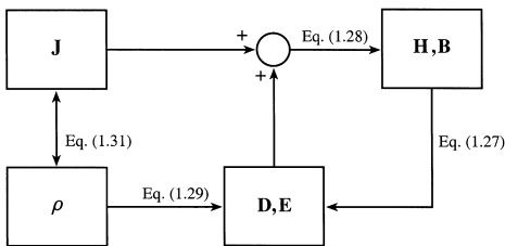
Figure 1.11 Generation of interdependent electric and magnetic fields, beginning with sources \mathbf{J} and \rho .
