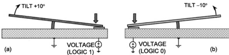
Figure 2.24 Simplified schematic of digital mirror device. Each pixel tilts \pm 10^\circ in response to applied voltages.
