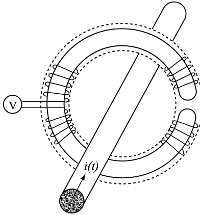
Figure 4.11 A method for measuring ac current in a conductor without inserting an ammeter into the circuit.
