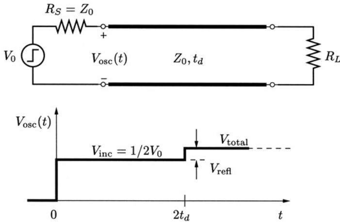
Figure 6.11 Illustration of the basic principle of time-domain reflectometry (TDR).
