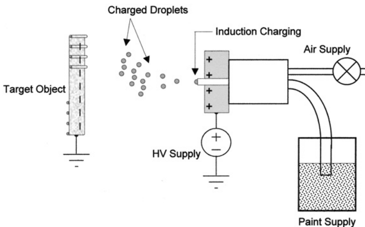
Figure 2.10 Basic electrostatic spray system. Droplets are charged by induction as they exit the atomization nozzle.
