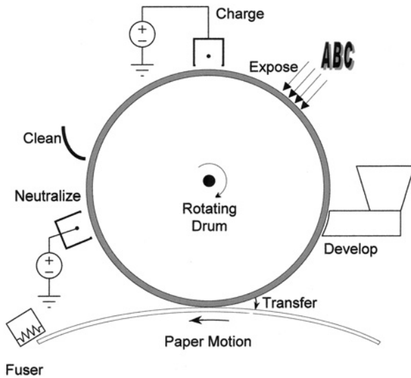
Figure 2.11 Basic elements of an electrostatic photocopier. As the light-sensitive drum rotates, it is charged, exposed to the image, dusted with toner, brought into contact with the paper, then discharged, and cleaned. The imprinted page passes through a fuser which melts the toner into the paper.
