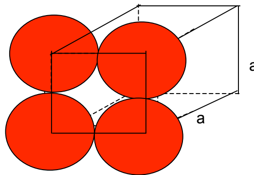
Figure 1.13: A simple cubic lattice showing relative positions of atoms on one face.
