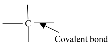
Figure 1.1 Carbon atom with its four bonds
