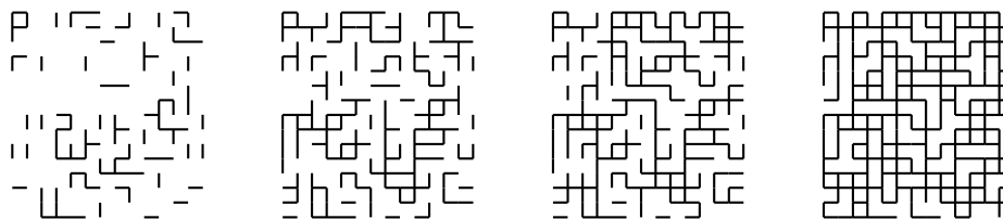
Figure 5 Bond-percolation configurations on a 14 \times 14 piece of the square lattice \mathbb{Z}^2 for p = 0.25 , p = 0.45 , p = 0.55 , p = 0.75 . The critical value is p_c = \frac{1}{2} .
