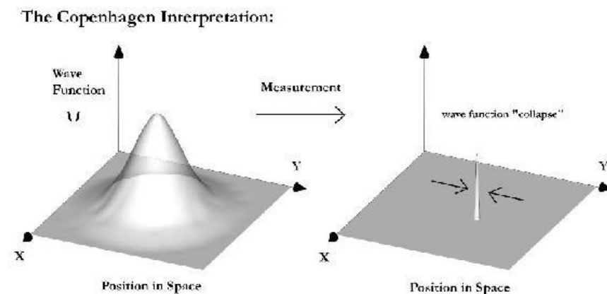
Figure 9: An example of the wave function collapse when observed. 74
