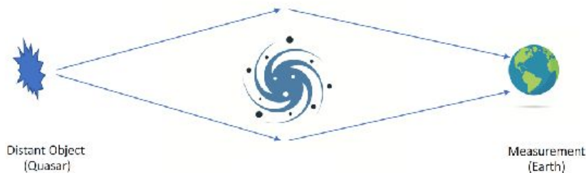
Figure 17: The cosmic delayed-choice experiment. 94
