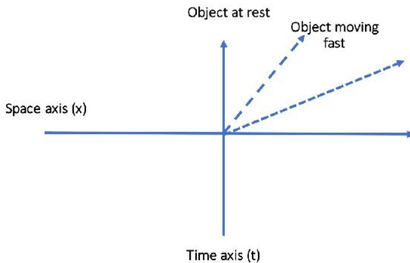
Figure 12: Simple space-time diagram with moving objects.
