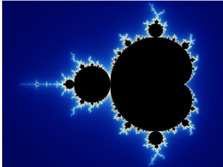
115 Figure 35: The Mandelbrot set.
