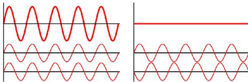
Figure 11: Example of Constructive (left side) and Destructive Interference (right side) 86
