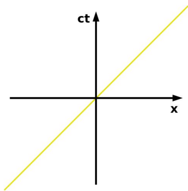
Figure 43: The format of a Minkowski space-time diagram.
