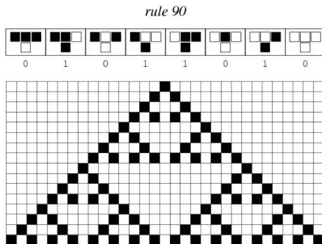
Figure 31: An example of running rule 90 in an elementary CA.
