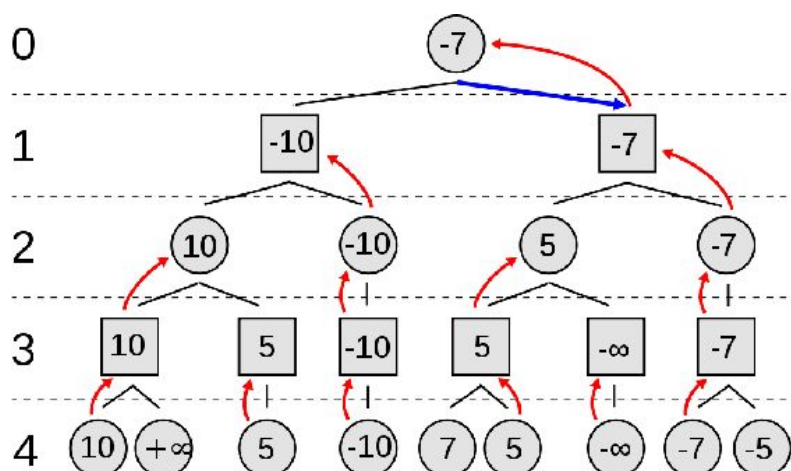
Figure 50: Minimax algorithm - an example of a simple game playing algorithm 143
