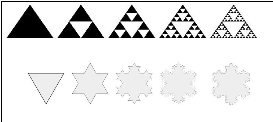
Figure 34: The Sierpinski Triangle and Koch Snowflake, examples of geometric fractals. 114
