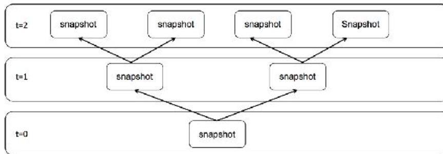
Figure 18: Example of snapshots above each other at time= t . 96
