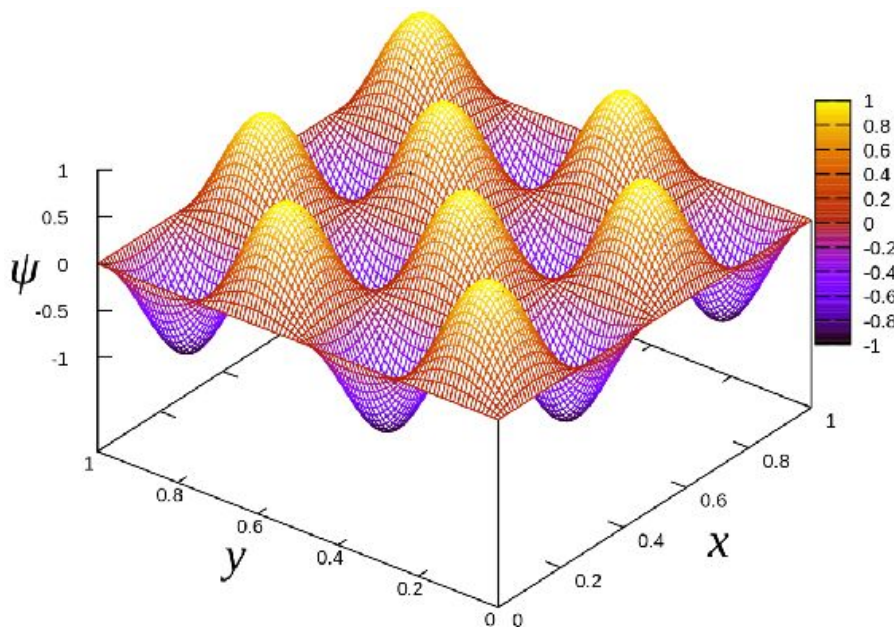
Figure 8: A graphical representation of a probability wave 73
