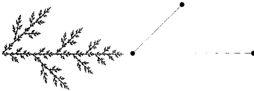
Figure 36: A random dendrite fractal pattern used to generate tree-like structures.
