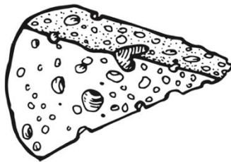
Figure 6: Bubbles in Swiss cheese is a way to visualize inflationary bubble universes. 59
