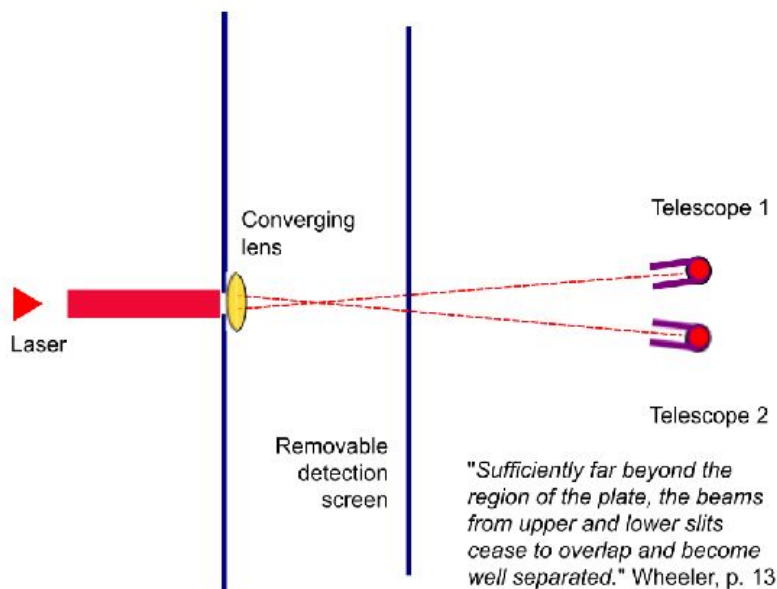
Figure 16: An example of Wheeler's delayed-choice, double-slit experiment. 92
