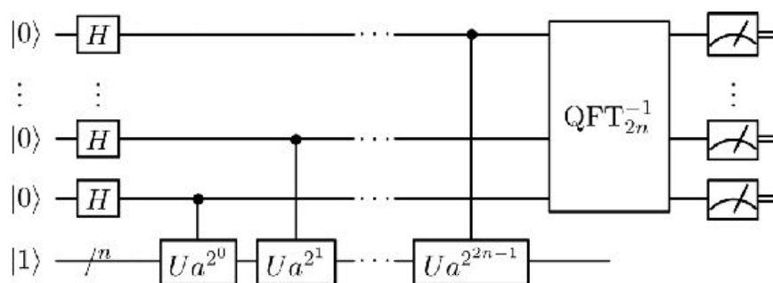
Figure 39: Shor's algorithm circuit diagram.
