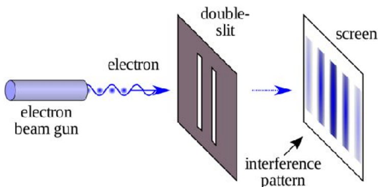
Figure 7: The double-slit experiment that shows that electrons behave as waves or as particle. 70
