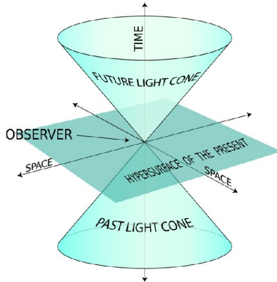
Figure 13: Space-time diagram with light cones for future and past events reachable by light. 89
