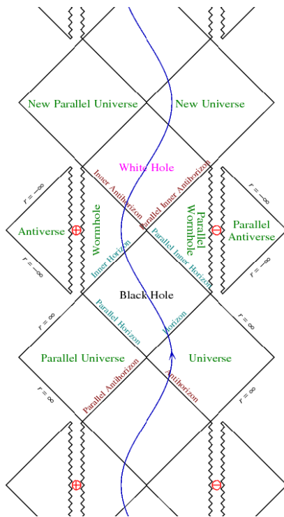
Figure 4: A Penrose diagram depicts the parallel worlds that might be reached via a rotating black hole. 54
