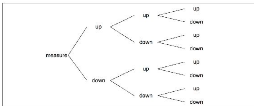
Figure 10: An example of the multiple measurements and how they would result in many worlds.
