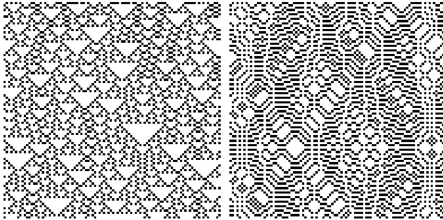
Figure 32: Comparison of Rule 18 and Rule 18R, using second-order rules.
