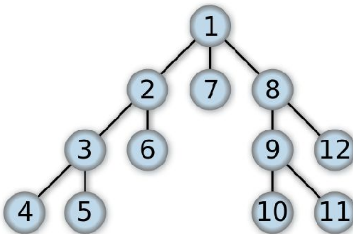
Figure 52: Example of depth-first search.
