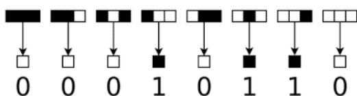
Figure 30: An example of a rule set consisting of 8 sub-rules.
