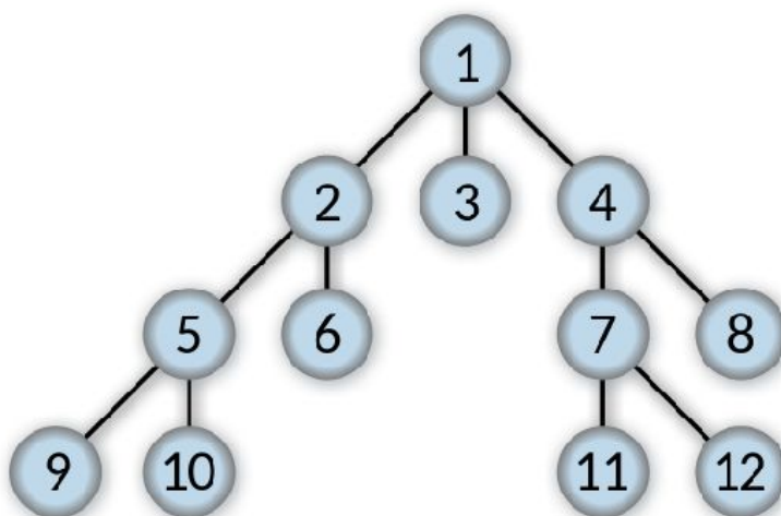
Figure 51: A breadth-first search of the graph. The numbers represent the order in which nodes are evaluated.
