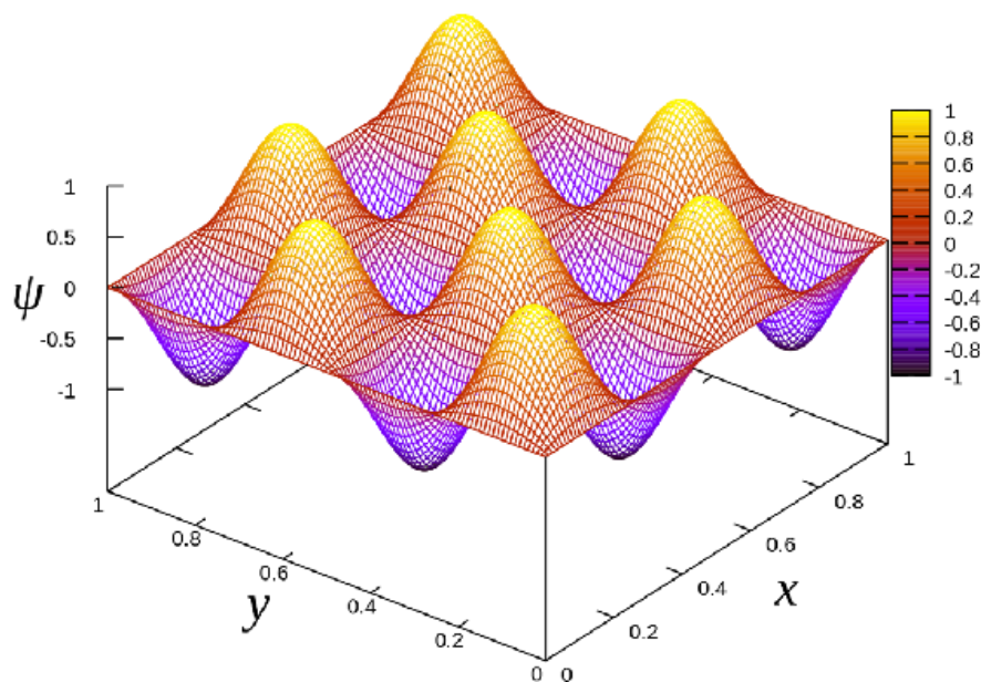
Figure 18: This is an example of a probability wave for a particle. 25
