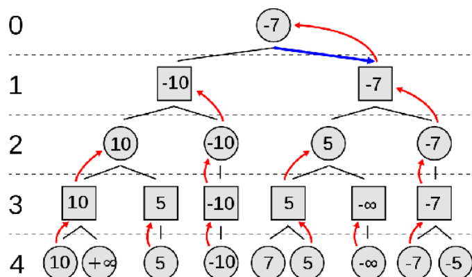
Figure 24: The minimax algorithm: a simple AI for evaluating future outcomes and choosing the best path. 34
