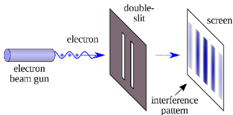
Figure 19: The double slit experiment with electrons showing an interference pattern 26
