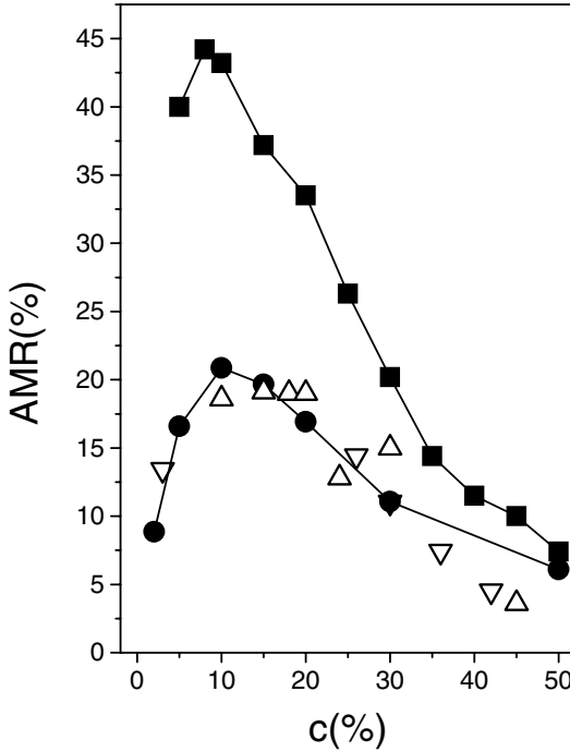
Fig. 26.19. Calculated and experimental AMR ratios of \text{Ni}_{1-c}\text{Fe}_c alloys. Full circles: see [18] full squares: see [19]; up-triangles: experiment, see [20]; down-triangles: experiment, see [21] and [22].
