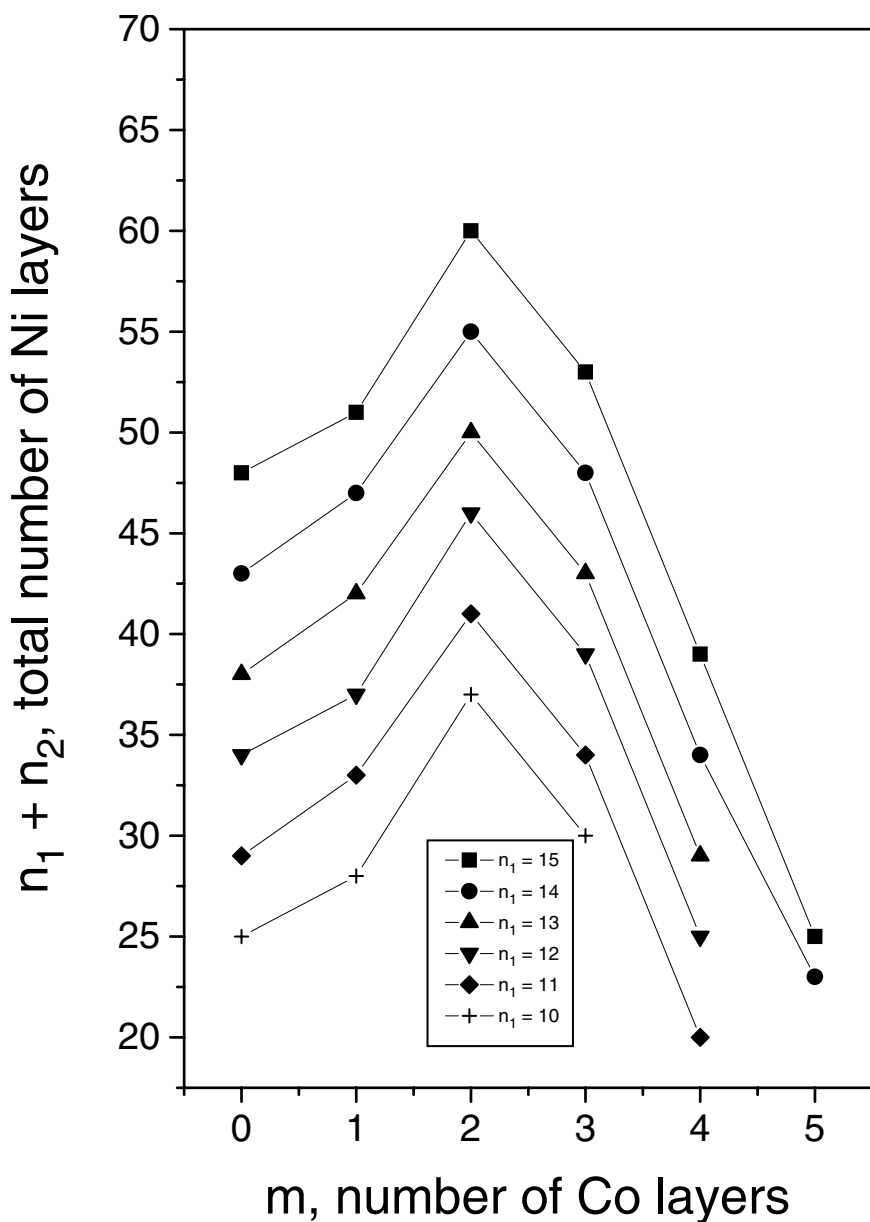
Fig. 26.12. Total number of Ni layers ( n_1 + n_2 ) at which the magnetic anisotropy energy, \Delta E_a of Cu(100)/Ni _{n_1} (-5.5%)/Ni _{n_2} (0%)/Co _m changes sign, displayed as a function of the number of Co layers ( m ). From [15].
