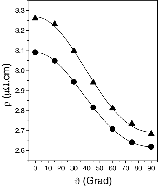
Fig. 26.20. Calculated resistivities with respect to the the angle, \vartheta , between the current and the magnetization for \text{Ni}_{85}\text{Fe}_{15} (triangles) and \text{Ni}_{80}\text{Fe}_{20} (circles) alloys. Solid lines visualize the results of least square fits according to (26.38), see text.
