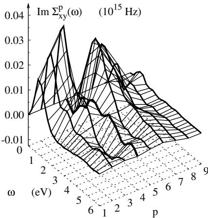
Fig. 26.29. Imaginary (absorptive) parts of the layer-resolved complex optical conductivity \Sigma_{\mu\nu}^p(\omega) for Pt 3 /Co/Pt 5 /Pt(111) as a function of the optical frequency \omega and the layer index p . The line at p = 4 refers to the Co layer-resolved optical conductivity. From [27].
