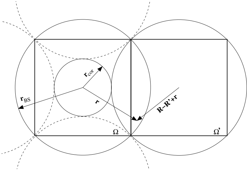
Fig. 20.3. Illustration of two near cells with overlapping bounding spheres. Dashed circles denote bounding spheres of other near cells. Also indicated is the radius r_{\text{cor}} outside which the near field corrections have to be calculated.
