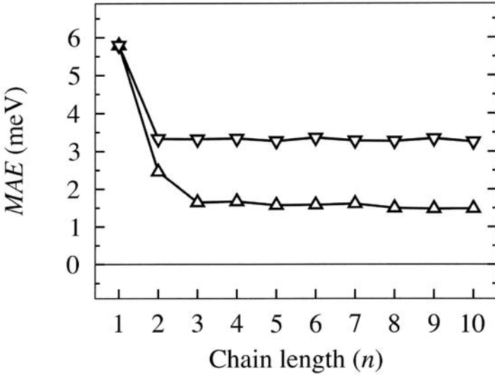
Fig. 26.16. Calculated magnetic anisotropy energies (MAE) for \text{Co}_n ( n = 1, \dots, 10 ) chains on Pt(111) including also contributions from nearest neighbor Pt sites and normalized to one Co atom. Up- and down triangles refer to \Delta E_{x-z} and \Delta E_{y-z} , respectively. From [16].
