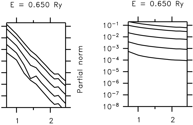
Fig. 17.1. Screened (left panel) and unscreened (right panel) partial norms for \ell = \ell' and \epsilon = 0.65 Ry as function of the distance in units of the lattice constant. The results for \ell = 0, 1, 2, 3, 4 are shown from top to bottom. From [5].
