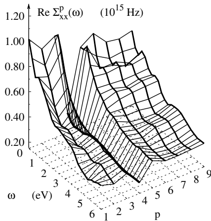
Fig. 26.28. Real (absorptive) parts of the layer-resolved complex optical conductivity \Sigma_{\mu\nu}^p(\omega) for Pt 3 /Co/Pt 5 /Pt(111) as a function of the optical frequency \omega and the layer index p . The line at p = 4 refers to the Co layer-resolved optical conductivity. From [27].
