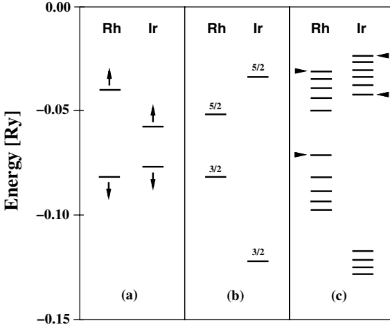
Fig. 14.3. Calculated positions of d-like resonances of a Rh and an Ir overlayer for the case of a Ag(001) substrate. The potentials from the scalar-relativistic spin-polarized calculations were used for the different single-site scattering schemes. Panel (a) refers to the scalar-relativistic spin-polarized case, where the spin-up and spin-down channels are denoted by up and down arrows. The relativistic non-magnetic case is shown in panel (b) illustrating the spin-orbit splitting between the j=3/2 and 5/2 resonances. The relativistic spin-polarized case is displayed in panel (c) and shows a total of ten different resonance energies for each case. The uncoupled resonances corresponding to (j, \mu) = (5/2, -5/2) (upper ones) and (5/2, 5/2) (lower ones) are indicated by small horizontal arrows. From [3].
