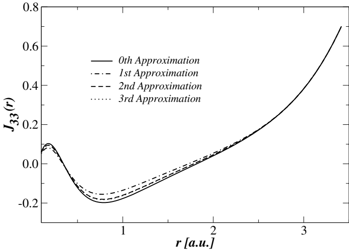
Fig. 6.2. Non-spherical components of irregular scattering solutions and their convergence with respect to various Born approximations for (bulk) fcc-Cu(100): J_{33}(r) at a complex energy below the Fermi energy.
