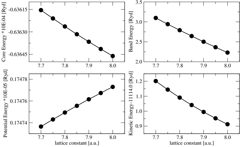
Fig. 22.4. Kinetic Energy and its separate contributions for Ag(100) versus the lattice parameter, \ell_{\max} = 4 .
