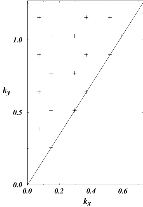
Fig. 18.6. Distribution of k points in the irreducible part of the Brillouin zone of a two-dimensional hexagonal lattice for a fcc or bcc (111) plane.
