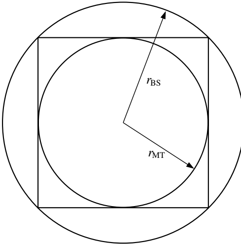
Fig. 4.1. Characteristic radii for a square lattice.
