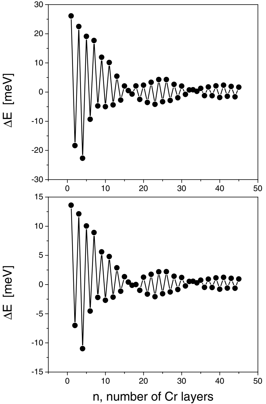
Fig. 26.6. Antiparallel (top) and perpendicular (bottom) interlayer exchange coupling in bcc-Fe(100)/Fe 6 Cr n Fe 6 /Vac. From [13].
