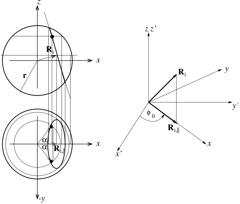
Fig. 4.2. Right part: The coordinate system is rotated around the z axis such that \mathbf{R}_{i,\parallel} points in x direction.
