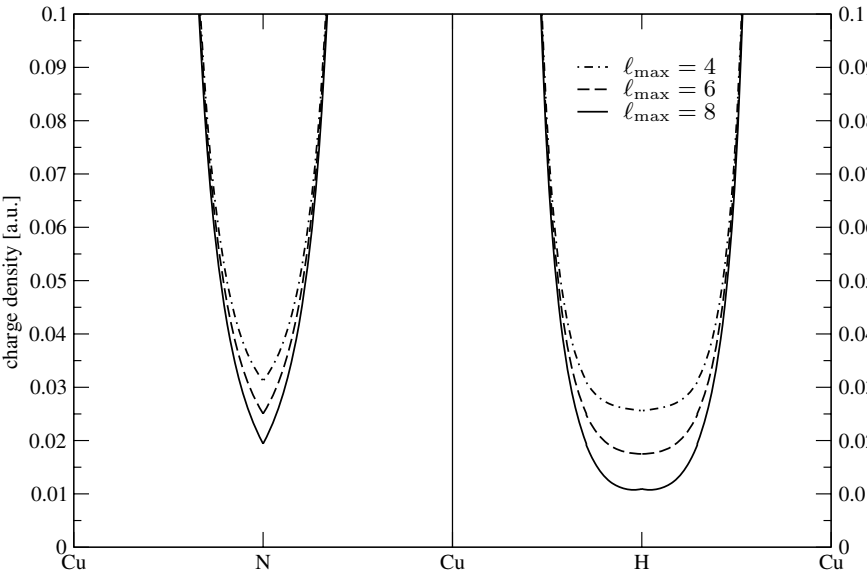
Fig. 21.4. Converged bulk Cu charge densities between three Coulomb singularities for three different \ell_{\max} for the potential. The label “H” marks a cell corner and “N” the center of a boundary plane.
