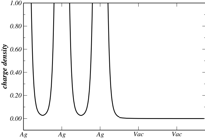
Fig. 26.1. Charge density of Ag (001) plotted along the nearest neighbor direction as indicated in Fig. 26.4.
