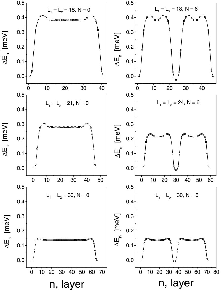
Fig. 26.35. Layer-resolved interlayer exchange or twisting energy for growing values of L . The various cases of L_1, L_2 and N are indicated. Note that the first and last three layers are the buffer layers. From [30].
