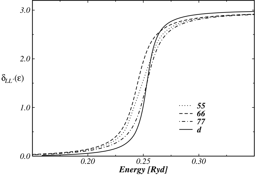
Fig. 14.1. Phase shifts in fcc-Ag for \ell = 2 (ASA calculation), and \ell = 2, m = -2, -1, 0 (full-potential calculation). The phase shift \delta_{\ell=2}(\varepsilon) is labelled by d , while \delta_{LL}(\varepsilon) is denoted by LL with the composite index L = (\ell, m) = \ell(\ell + 1) + m + 1 . Note that due to the symmetry of the system \delta_{55}(\varepsilon) = \delta_{99}(\varepsilon) and \delta_{66}(\varepsilon) = \delta_{88}(\varepsilon) , see also Table 14.1.
