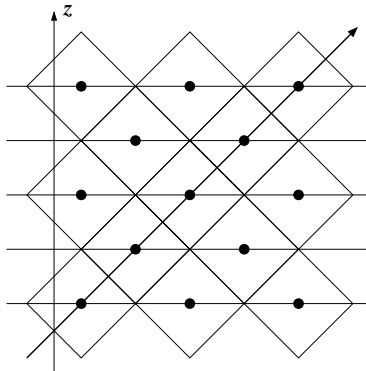
Fig. 26.4. Nearest neighbor direction for an fcc (001) surface.
