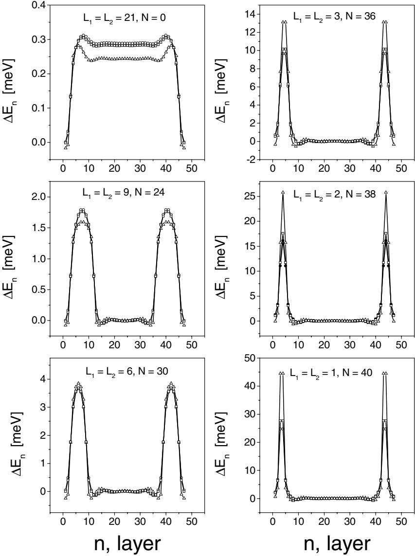
Fig. 26.34. Layer- and component-resolved interlayer exchange or twisting energy for L = 42 ML. The various cases of L_1, L_2 and N are indicated. Note that the first and last three layers refer to buffer layers. Circles and triangles refer to Ni and Fe, respectively, squares to the average. From [30].
