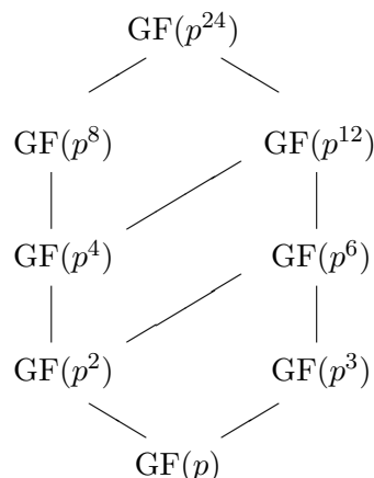
Figure 20.1. Subfields of \text{GF}(p^{24})
