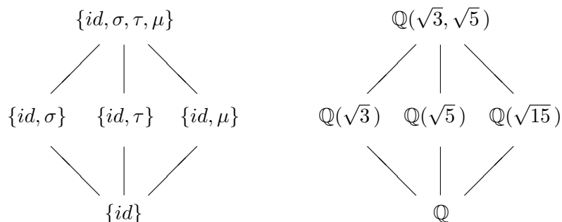
Figure 21.1. G(\mathbb{Q}(\sqrt{3}, \sqrt{5})/\mathbb{Q})
