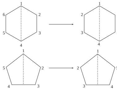
Figure 4.2. Rotations and reflections of a regular n -gon
