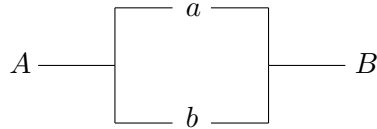
Figure 17.4. a \vee b
