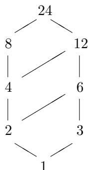
Figure 17.2. A partial order on the divisors of 24
