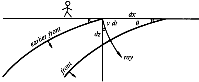
Figure 3.3: Downgoing fronts and rays in stratified medium v(z) . The wavefronts are horizontal translations of one another. dwnc-frontz [NR]
