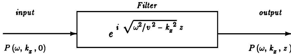
Figure 3.4: Downward continuation of a downgoing wavefield. dwnc-inout [NR]
