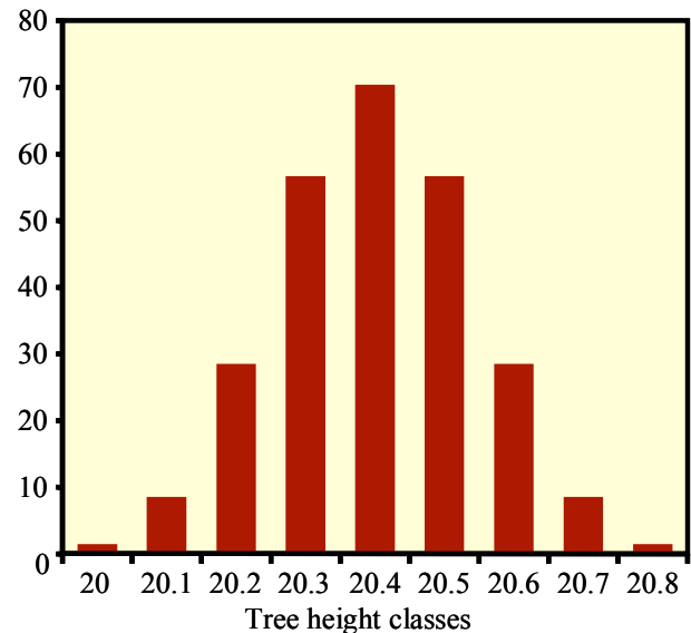
Segregation from the cross AaBbCcDd x AaBbCcDd , number
