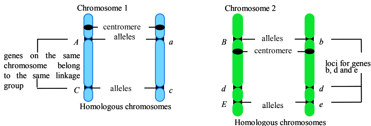
Figure 1-2. Two pairs of homologous chromosomes are shown. Genes with dominant alleles (capital letters) and genes with recessive alleles (small letters) located at loci in the same or different linkage groups are indicated.
