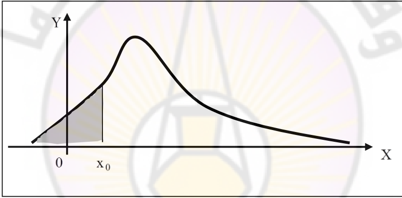
الشكل (8-26) F(x_0) = P(X \leq x_0)
