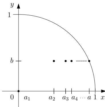
Figure 10.7: f is not continuous at (a, b) .
