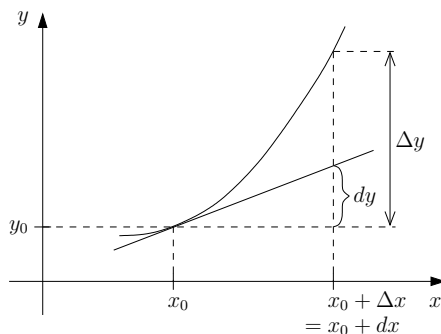
Figure 4.2: dy is the change in y along the tangent line.
